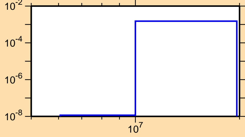
\sigma vs. E for ^{137}\text{Ce}(n,d)
