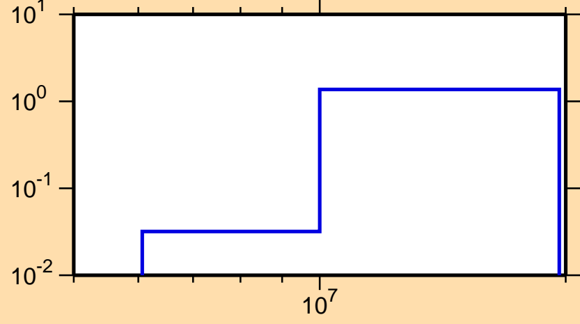
\sigma vs. E for ^{137}\text{Ce}(n,2n)
