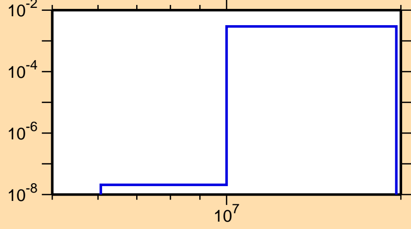
\sigma vs. E for ^{137}\text{Ce}(n,np)
