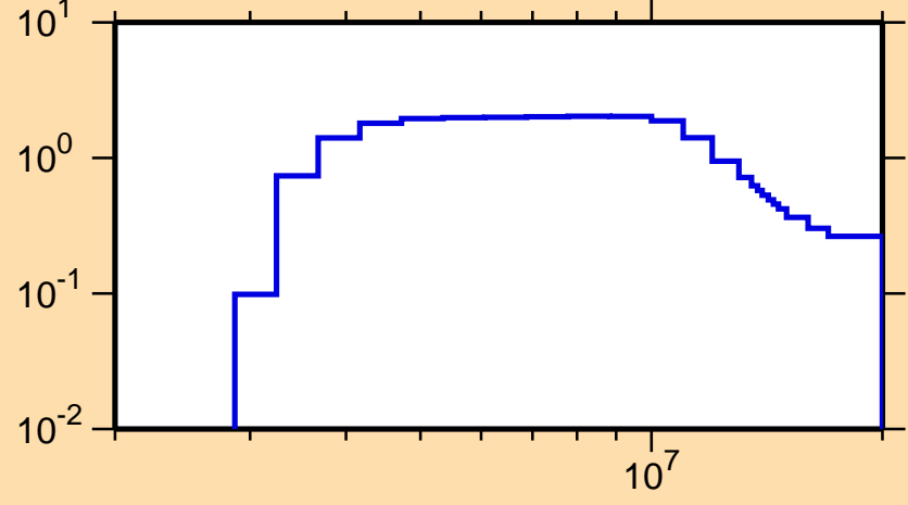
\sigma vs. E for ^{138}\text{Ce}(n,n\text{cont.})
