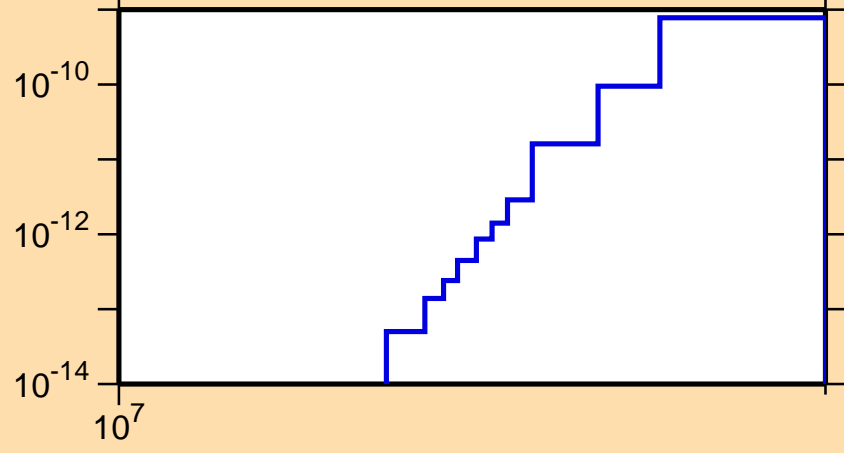
\sigma vs. E for ^{138}\text{Ce}(n,p\alpha)
