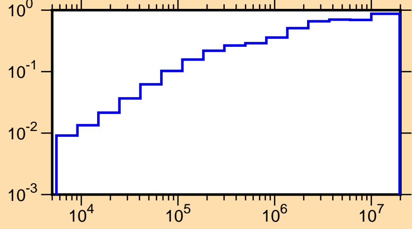
\mu vs. E for ^{138}\text{Ce}(\text{mt251})
