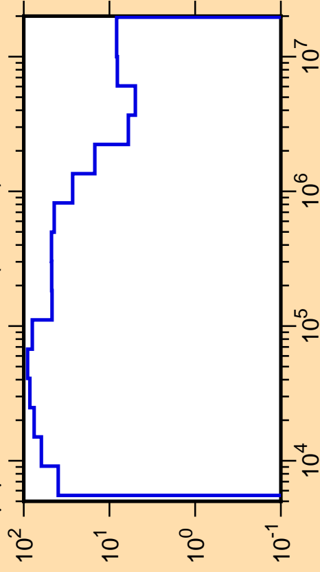
\Delta\mu/\mu vs. E for ^{138}\text{Ce}(\text{mt251})
