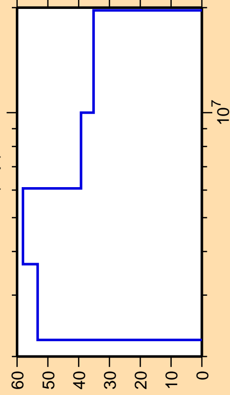
\Delta\sigma/\sigma vs. E for ^{138}\text{Ce}(n,p)
