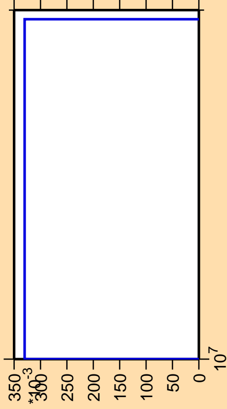
\Delta\sigma/\sigma vs. E for ^{138}\text{Ce}(n,pd)
