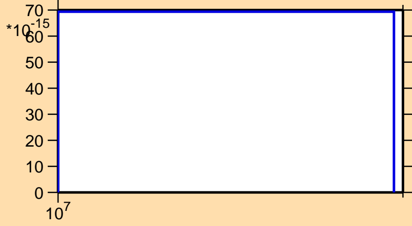
\sigma vs. E for ^{138}\text{Ce}(n,pd)
