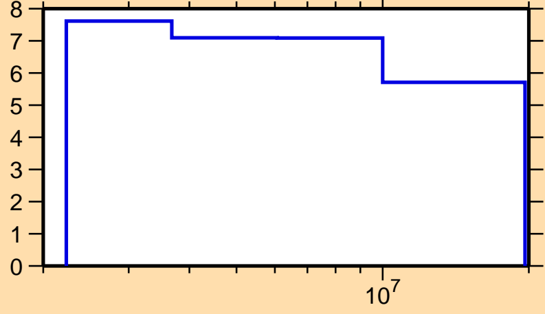
\Delta\sigma/\sigma vs. E for ^{138}\text{Ce}(n,n\text{onel.})
