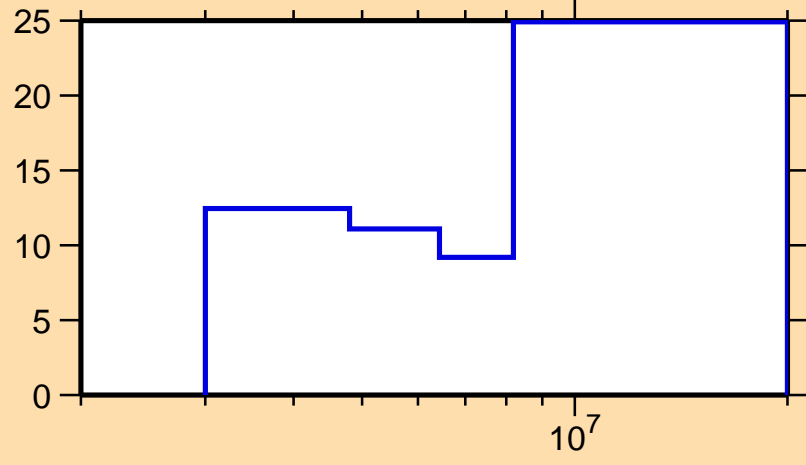
\Delta\sigma/\sigma vs. E for ^{138}\text{Ce}(n,n\text{cont.})
