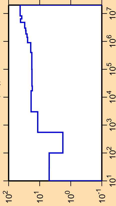
\Delta\sigma/\sigma vs. E for ^{138}\text{Ce}(n,\gamma)
