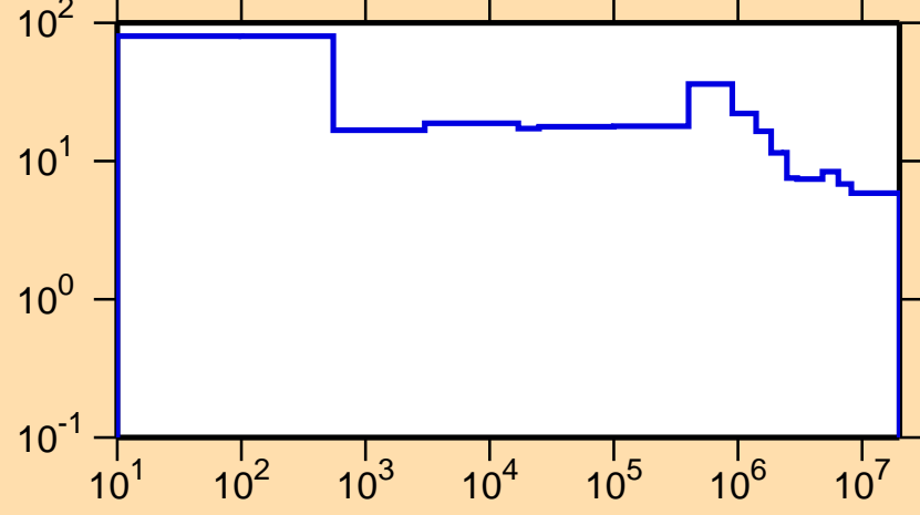
\Delta\sigma/\sigma vs. E for ^{138}\text{Ce}(n,\text{nonel.})
