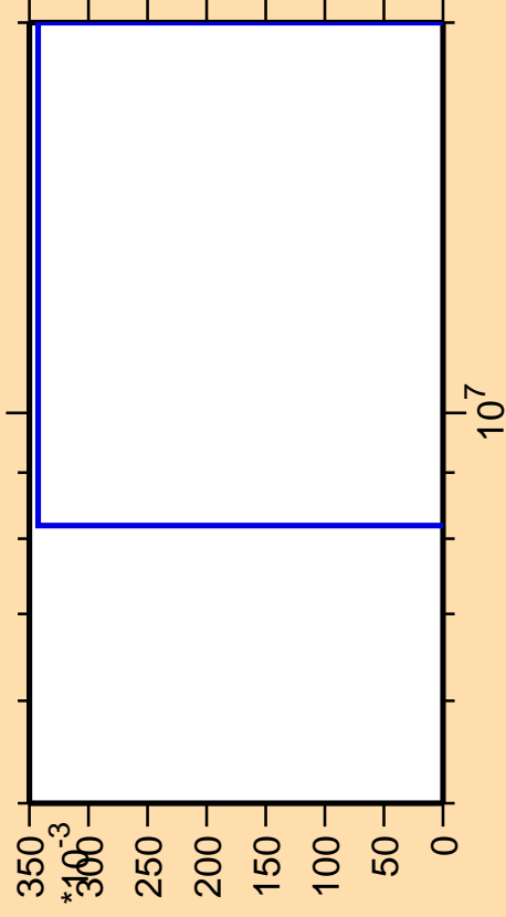
\Delta\sigma/\sigma vs. E for ^{138}\text{Ce}(n,\text{nt})
