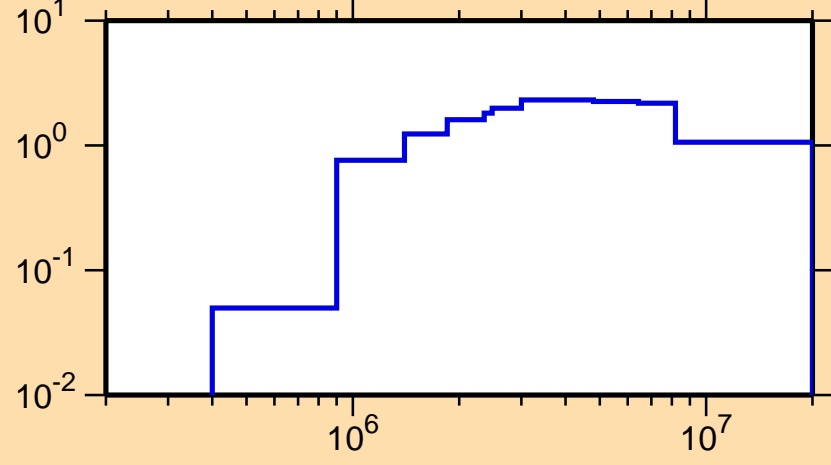
\sigma vs. E for ^{138}\text{Ce}(n,\text{inel.})
