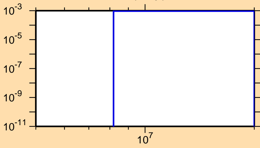
\sigma vs. E for ^{138}\text{Ce}(n,np)
