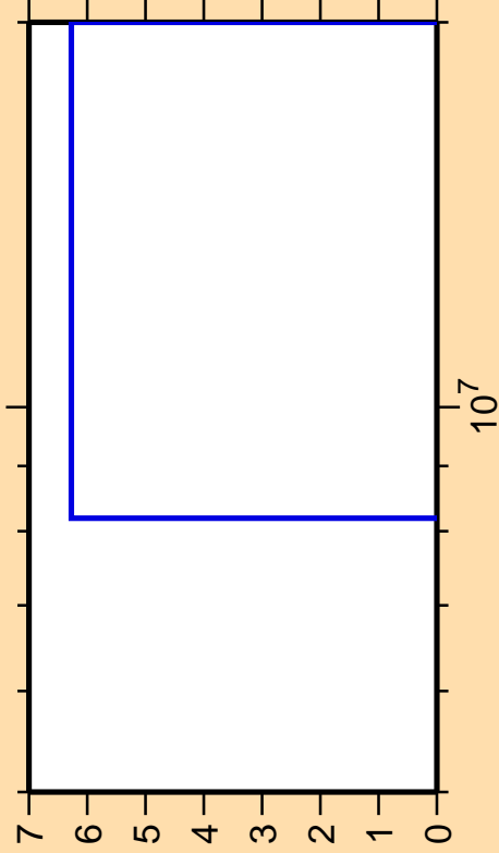
\Delta\sigma/\sigma vs. E for ^{138}\text{Ce}(n,2np)
