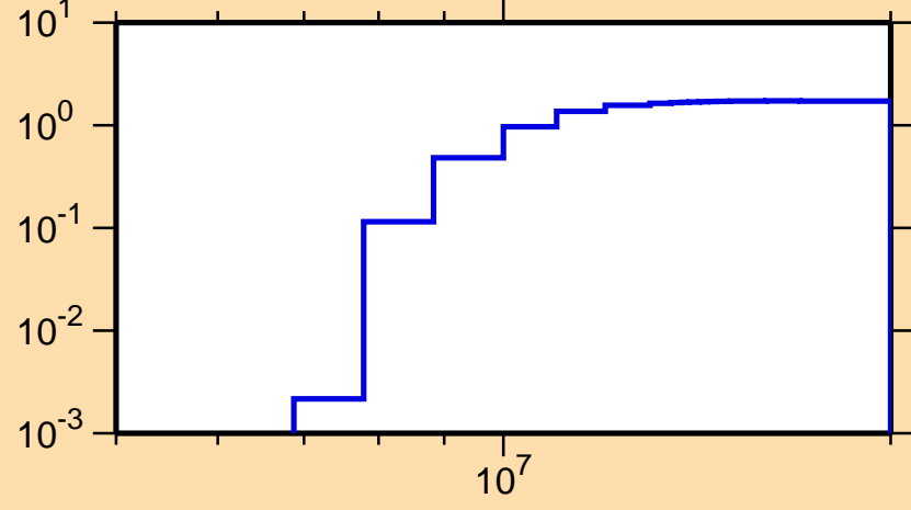
\sigma vs. E for ^{139}\text{Ce}(n,2n)
