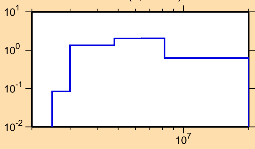
\sigma vs. E for ^{139}\text{Ce}(n,n\text{cont.})
