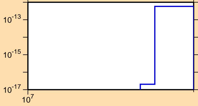
\sigma vs. E for ^{139}\text{Ce}(n,\text{pt})
