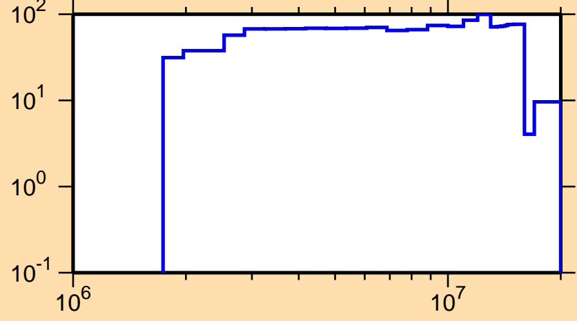
\Delta\sigma/\sigma vs. E for ^{139}\text{Ce}(n,n_1)
