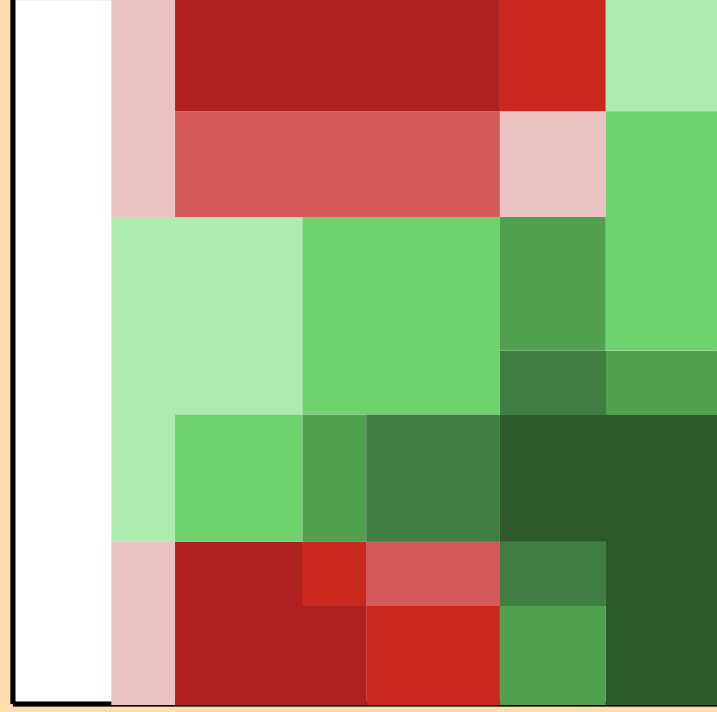
\Delta\sigma/\sigma vs. E for ^{139}\text{Ce}(n,2n)
