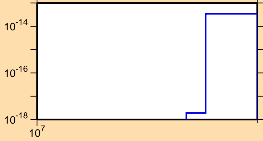
\sigma vs. E for ^{139}\text{Ce} (mt 34)
