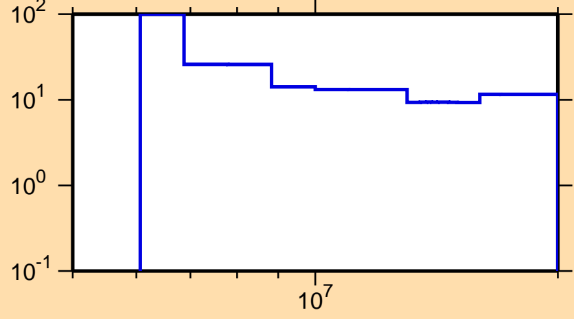
\Delta\sigma/\sigma vs. E for ^{139}\text{Ce}(n,2n)
