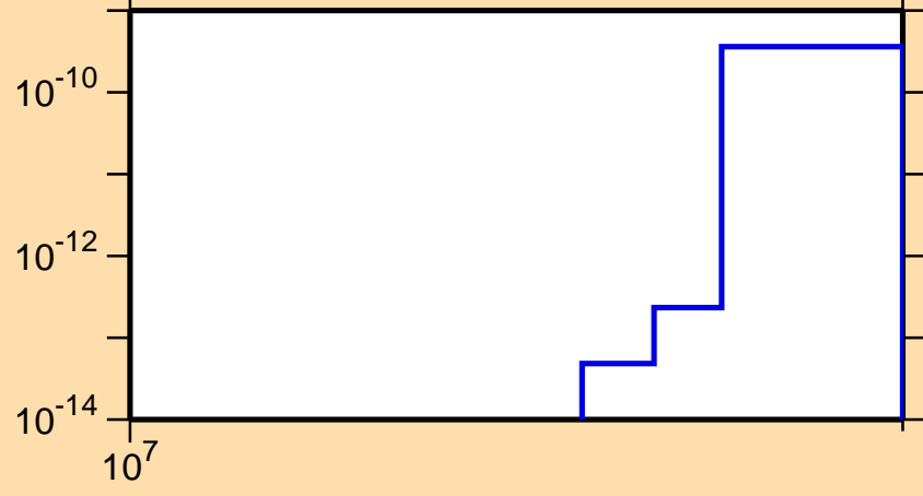
\sigma vs. E for ^{139}\text{Ce}(n,\text{nt})
