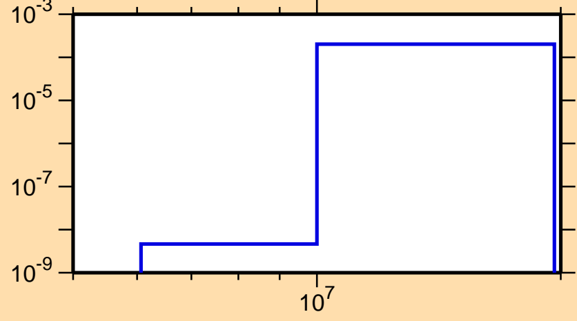
\sigma vs. E for ^{139}\text{Ce}(n,\alpha)
