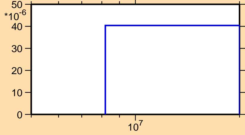
\sigma vs. E for ^{139}\text{Ce}(n,t)
