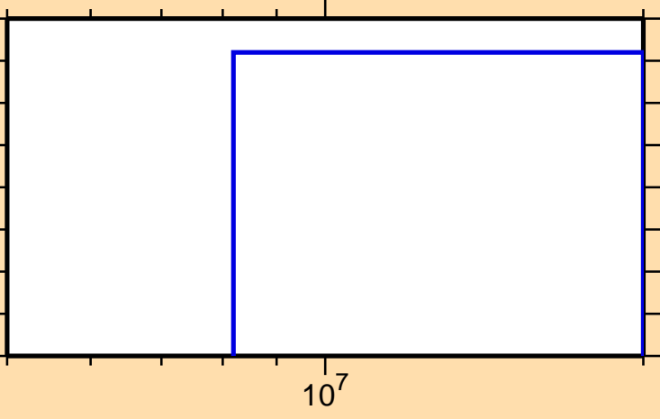
\sigma vs. E for ^{139}\text{Ce}(n,\text{He}3)
