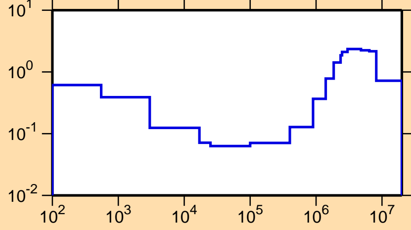
\sigma vs. E for ^{139}\text{Ce}(n,\text{inel.})
