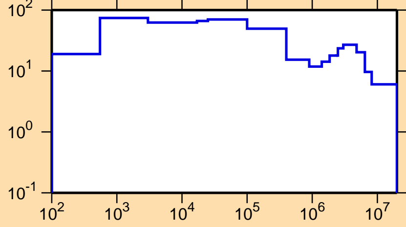
\Delta\sigma/\sigma vs. E for ^{139}\text{Ce}(n,\text{el.})
