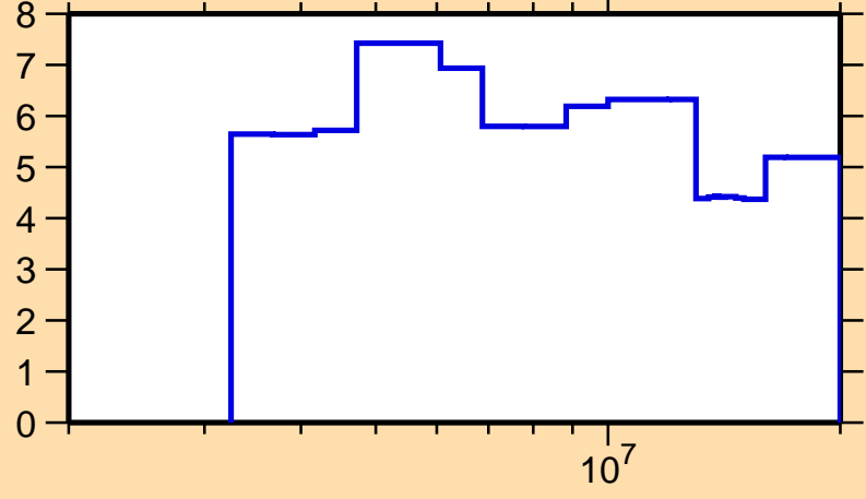
\Delta\sigma/\sigma vs. E for ^{140}\text{Ce}(n,\text{nonel.})
