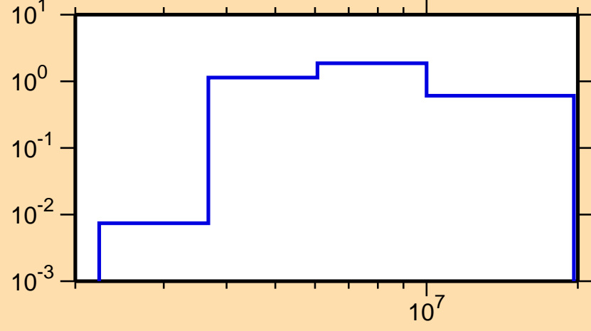
\sigma vs. E for ^{140}\text{Ce}(n,n\text{cont.})
