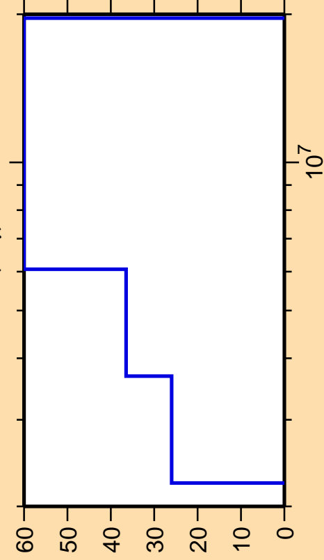
\Delta\sigma/\sigma vs. E for ^{140}\text{Ce}(n,\gamma)
