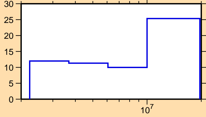
\Delta\sigma/\sigma vs. E for ^{140}\text{Ce}(n,n\text{cont.})
