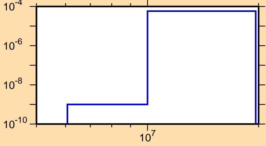
\sigma vs. E for ^{140}\text{Ce}(n,n\alpha)
