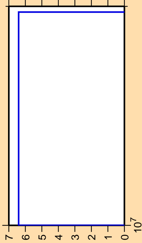
\Delta\sigma/\sigma vs. E for ^{140}\text{Ce}(n,2n\alpha)
