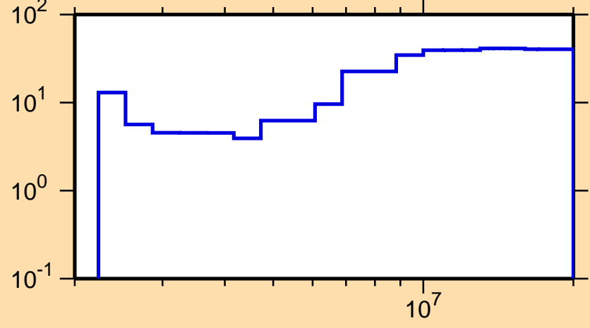
\Delta\sigma/\sigma vs. E for ^{141}\text{Ce}(n,\text{inel.})
