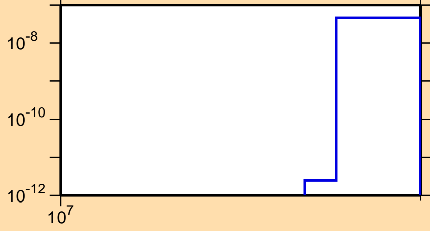
\sigma vs. E for ^{141}\text{Ce}(n,nt)
