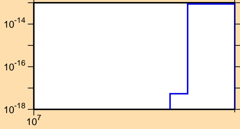
\sigma vs. E for ^{141}\text{Ce} (mt 34)
