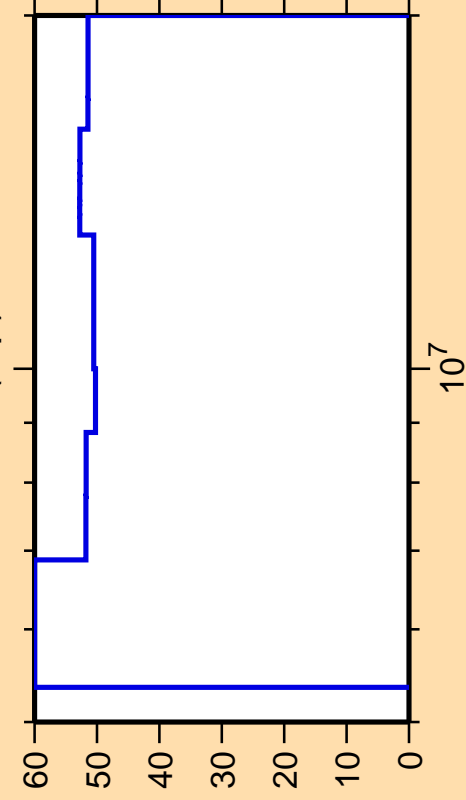
\Delta\sigma/\sigma vs. E for ^{141}\text{Ce}(n,p)
