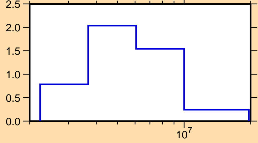
\sigma vs. E for ^{141}\text{Ce}(n,n\text{cont.})
