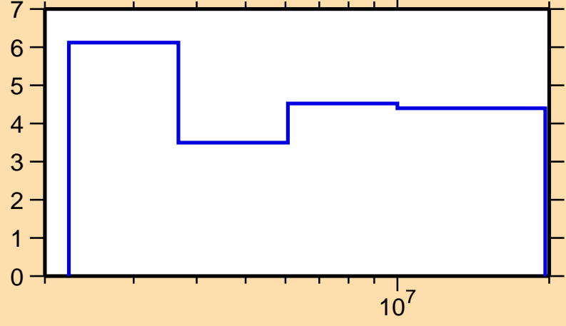
\Delta\sigma/\sigma vs. E for ^{141}\text{Ce}(n,\text{nonel.})
