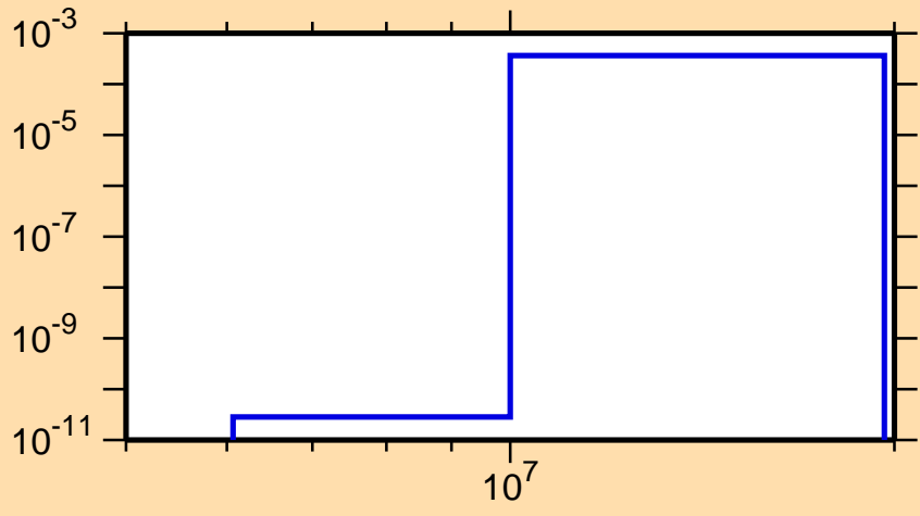
\sigma vs. E for ^{141}\text{Ce}(n,d)
