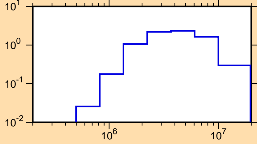
\sigma vs. E for ^{141}\text{Ce}(n,\text{inel.})
