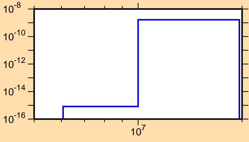
\sigma vs. E for ^{141}\text{Ce}(n,p\alpha)
