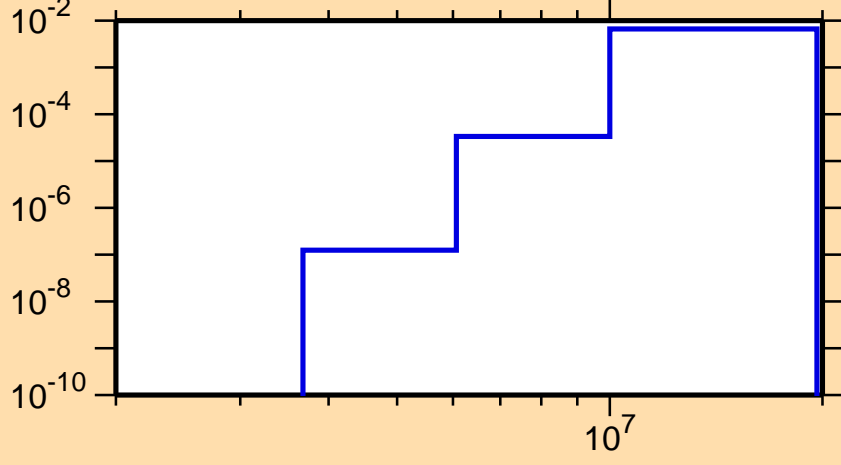
\sigma vs. E for ^{141}\text{Ce}(n,p)
