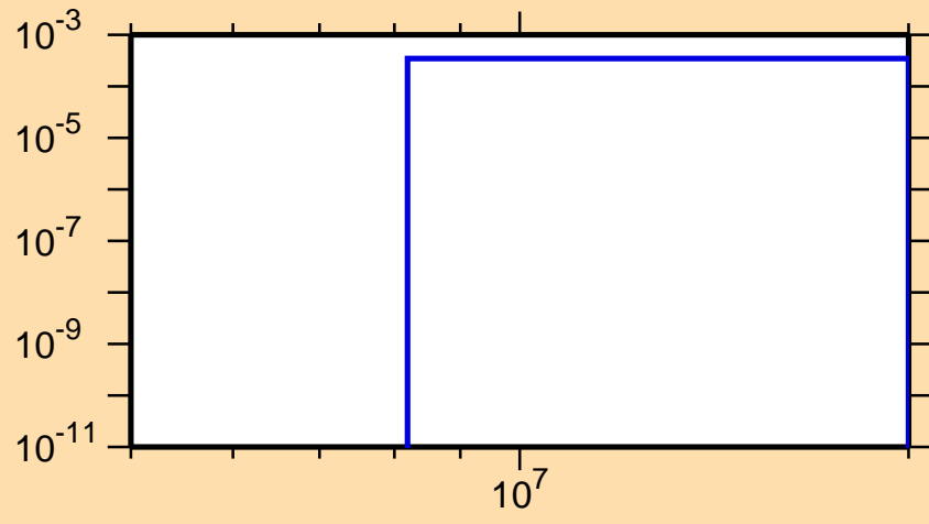
\sigma vs. E for ^{141}\text{Ce}(n,t)
