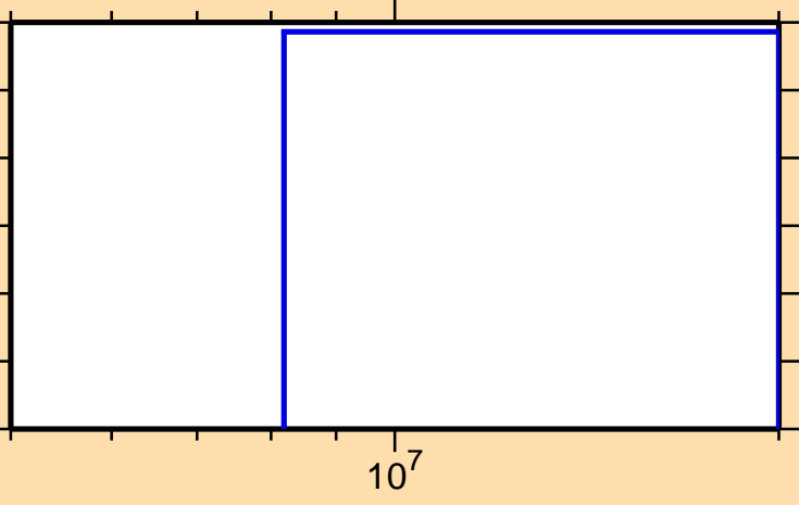
\sigma vs. E for ^{141}\text{Ce}(n,d)
