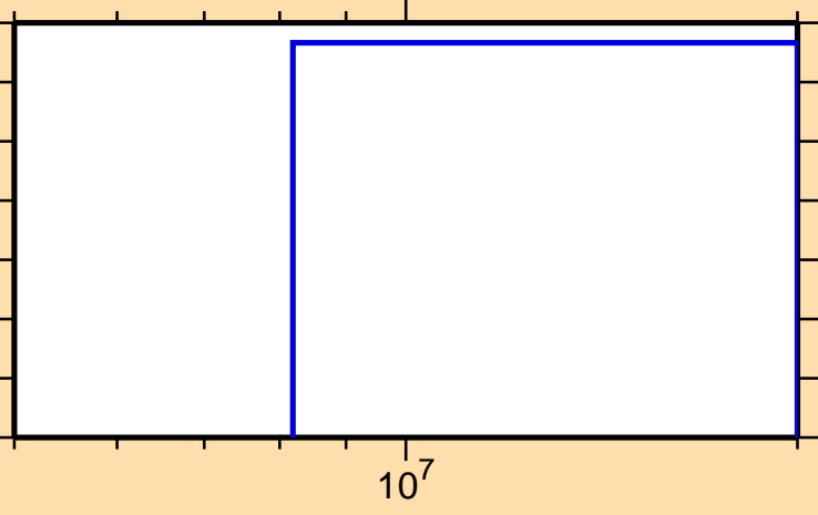
\sigma vs. E for ^{141}\text{Ce}(n,p\alpha)
