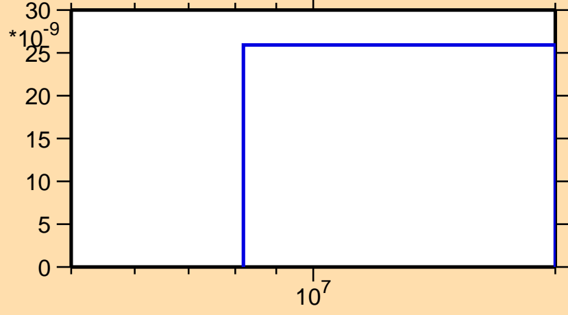
\sigma vs. E for ^{141}\text{Ce}(n,2np)
