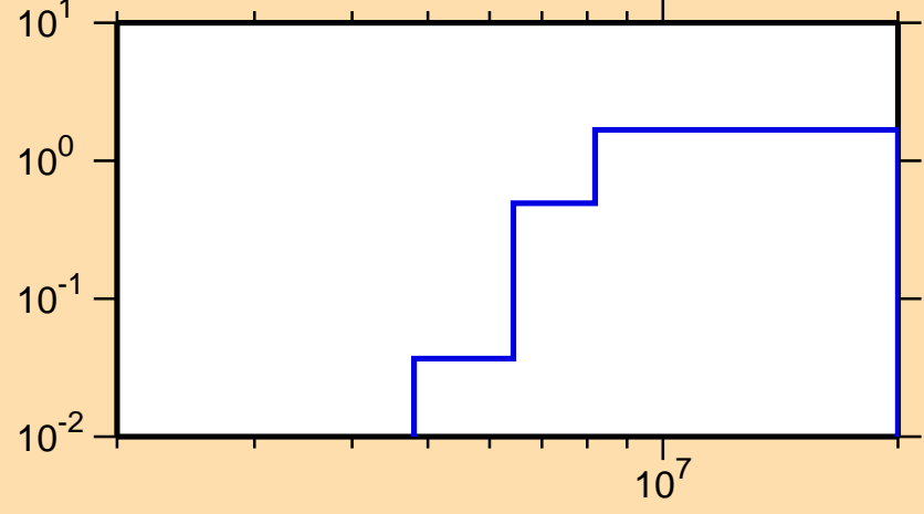
\sigma vs. E for ^{141}\text{Ce}(n,2n)
