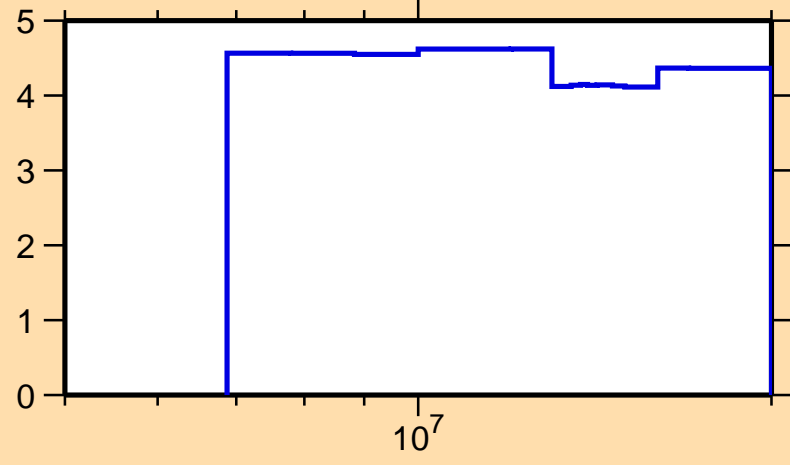
\Delta\sigma/\sigma vs. E for ^{142}\text{Ce}(n,\text{nonel.})
