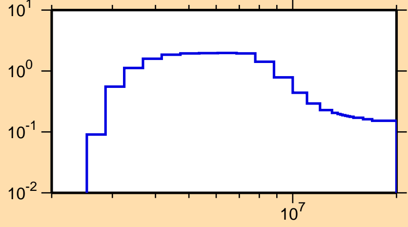
\sigma vs. E for ^{142}\text{Ce}(n,n\text{cont.})
