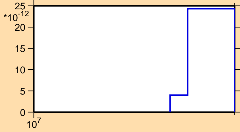
\sigma vs. E for ^{142}\text{Ce}(n,p\alpha)
