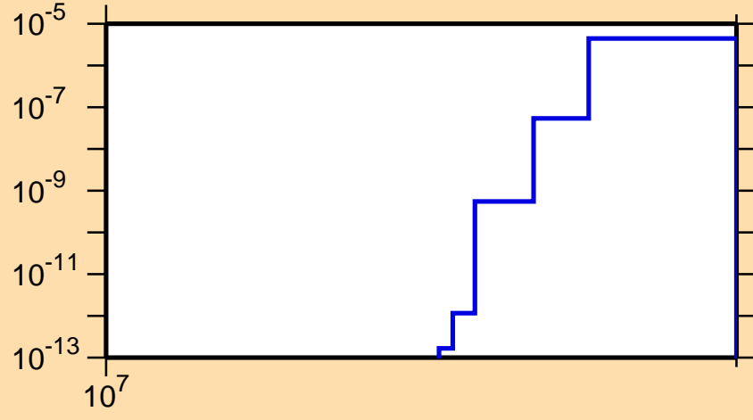
\sigma vs. E for ^{142}\text{Ce}(n,nt)
