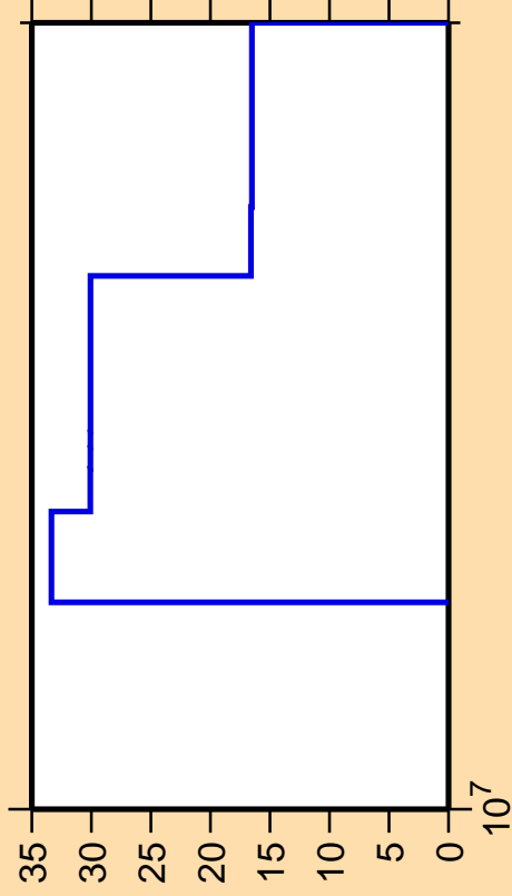
\Delta\sigma/\sigma vs. E for ^{142}\text{Ce}(n,3n)
