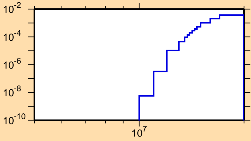
\sigma vs. E for ^{142}\text{Ce}(n,d)
