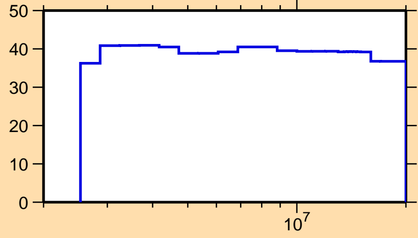
\Delta\sigma/\sigma vs. E for ^{142}\text{Ce}(n, n_1)
