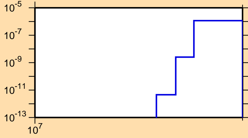
\sigma vs. E for ^{142}\text{Ce}(n,\text{nd})
