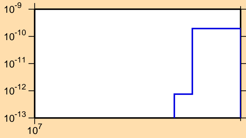
\sigma vs. E for ^{142}\text{Ce}(n,\text{He}3)
