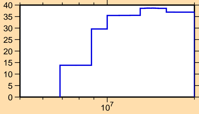
\Delta\sigma/\sigma vs. E for ^{142}\text{Ce}(n,\text{inel.})
