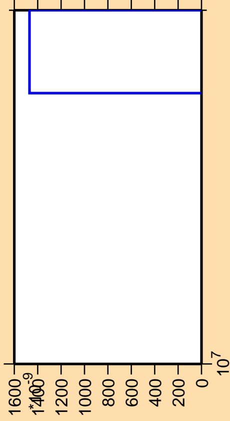
\Delta\sigma/\sigma vs. E for ^{142}\text{Ce} (mt 11)
