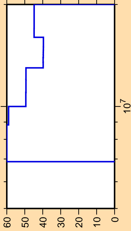
\Delta\sigma/\sigma vs. E for ^{142}\text{Ce}(n,p)
