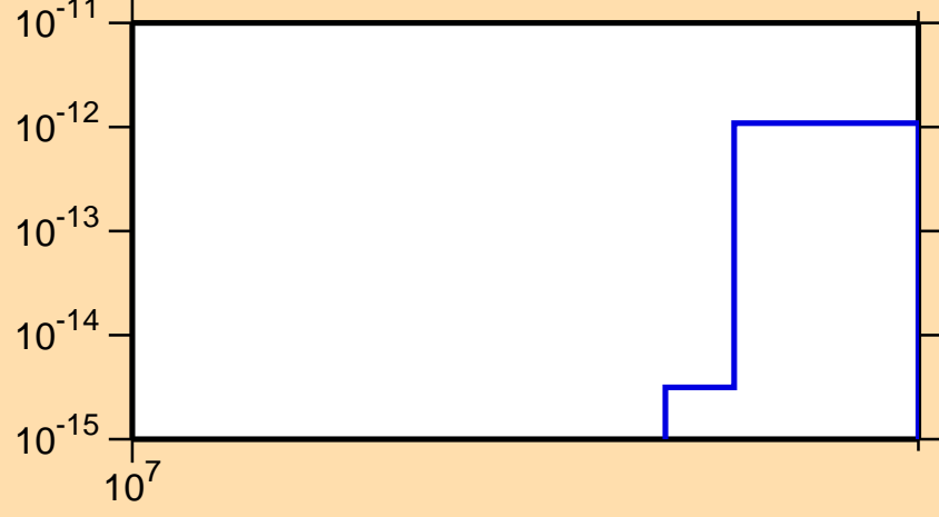
\sigma vs. E for ^{142}\text{Ce} (mt 45)
