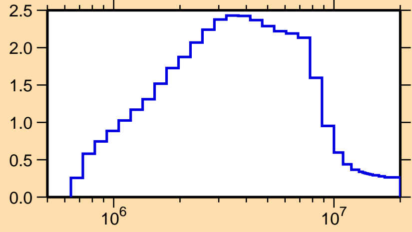
\sigma vs. E for ^{142}\text{Ce}(n,\text{inel.})
