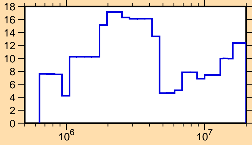
\Delta\sigma/\sigma vs. E for ^{142}\text{Ce}(n,\text{el.})
