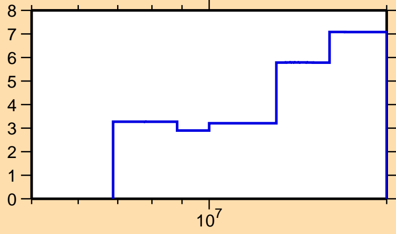
\Delta\sigma/\sigma vs. E for ^{142}\text{Ce}(n,\text{tot.})
