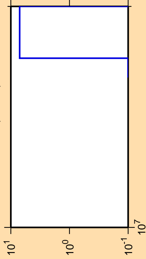
\Delta\sigma/\sigma vs. E for ^{142}\text{Ce} (mt 45)
