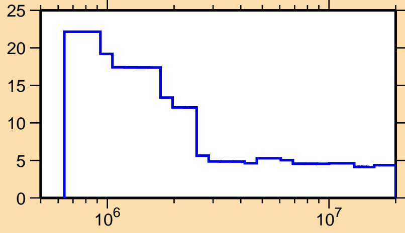
\Delta\sigma/\sigma vs. E for ^{142}\text{Ce}(n,\text{nonel.})
