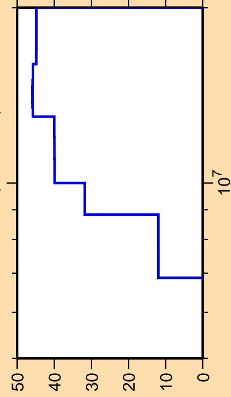
\Delta\sigma/\sigma vs. E for ^{142}\text{Ce}(n,n\text{cont.})
