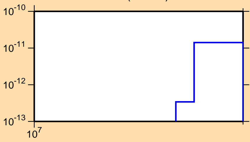
\sigma vs. E for ^{142}\text{Ce}(\text{mt117})
