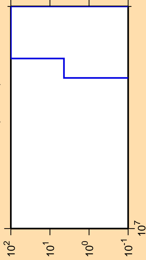
\Delta\sigma/\sigma vs. E for ^{142}\text{Ce}(n,\text{He}3)
