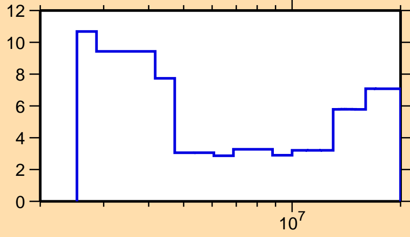
\Delta\sigma/\sigma vs. E for ^{142}\text{Ce}(n,\text{tot.})
