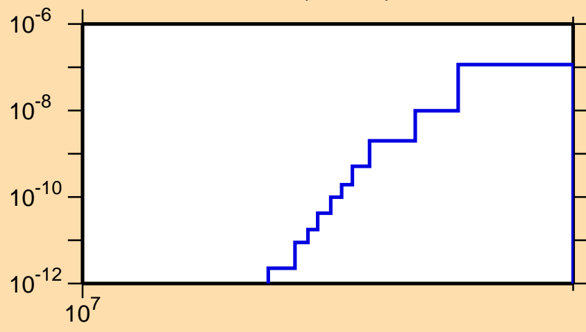
\sigma vs. E for ^{142}\text{Ce}(n,2n\alpha)
