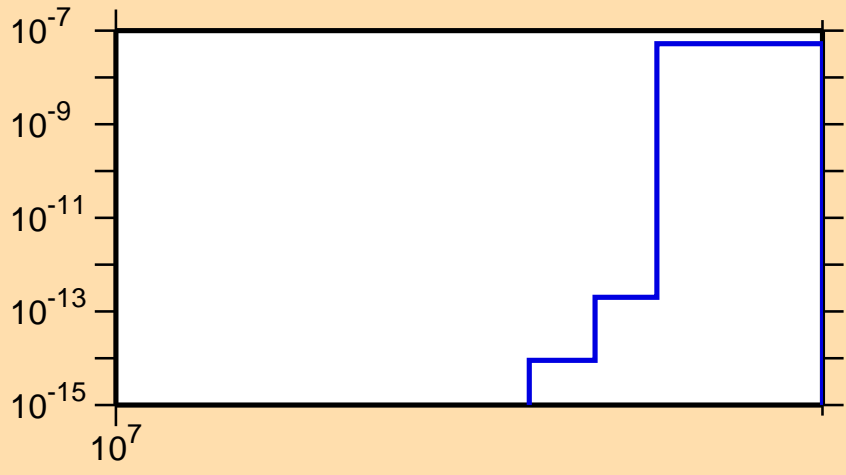
\sigma vs. E for ^{142}\text{Ce}(n,2np)
