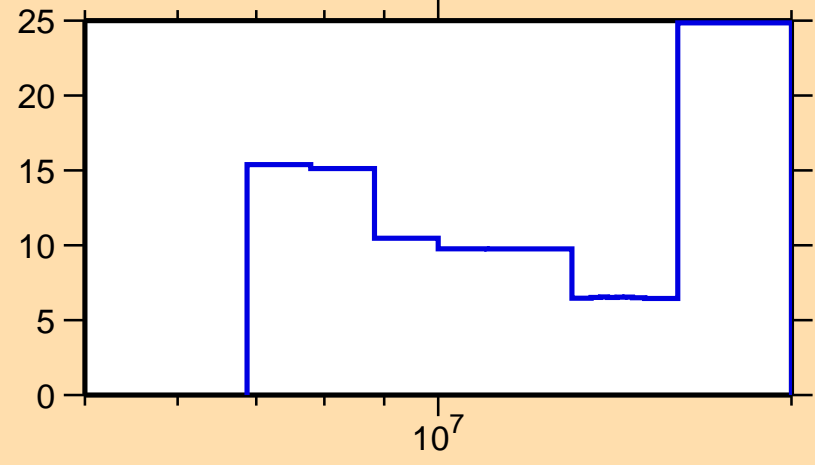
\Delta\sigma/\sigma vs. E for ^{142}\text{Ce}(n,2n)
