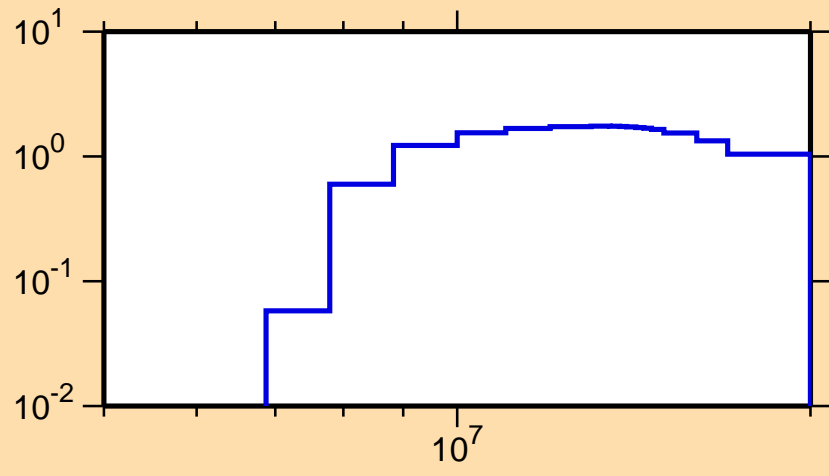
\sigma vs. E for ^{142}\text{Ce}(n,2n)
