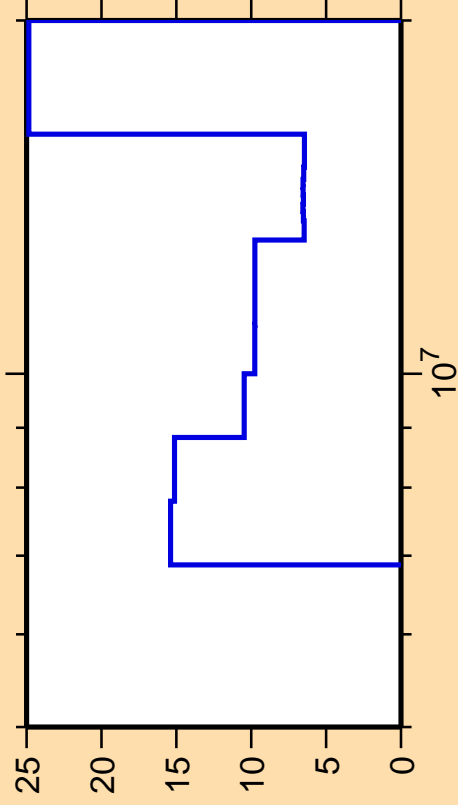
\Delta\sigma/\sigma vs. E for ^{142}\text{Ce}(n,2n)
