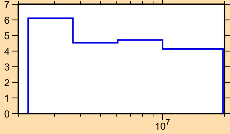
\Delta\sigma/\sigma vs. E for ^{142}\text{Ce}(n,\text{nonel.})
