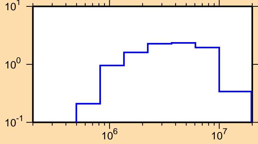
\sigma vs. E for ^{142}\text{Ce}(n,\text{inel.})
