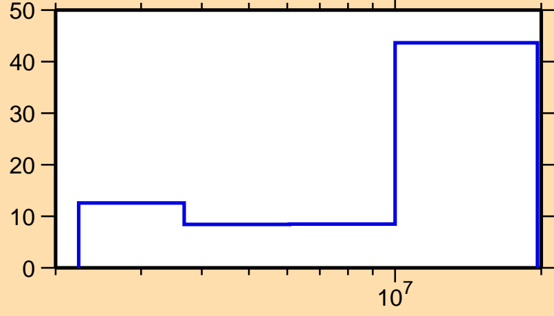
\Delta\sigma/\sigma vs. E for ^{142}\text{Ce}(n,n\text{cont.})
