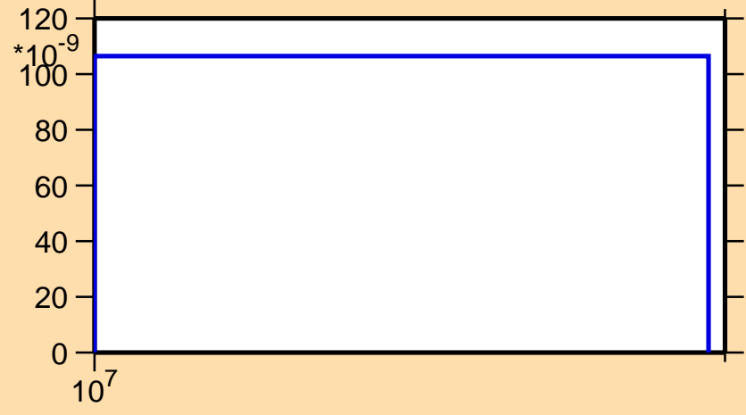
\sigma vs. E for ^{143}\text{Ce}(n,\text{nd})
