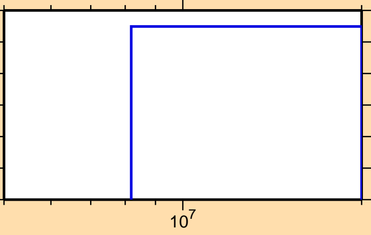
\sigma vs. E for ^{143}\text{Ce}(n,nt)
