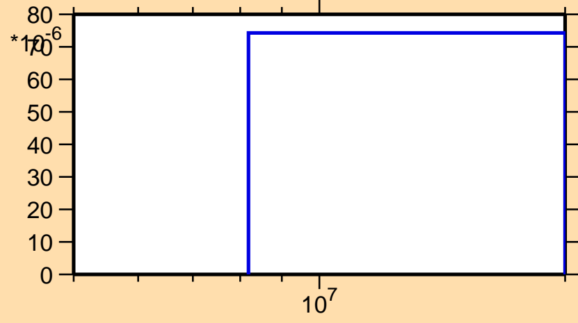
\sigma vs. E for ^{143}\text{Ce}(n,np)
