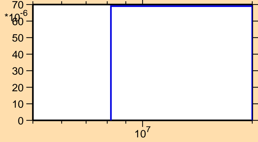
\sigma vs. E for ^{143}\text{Ce}(n,t)
