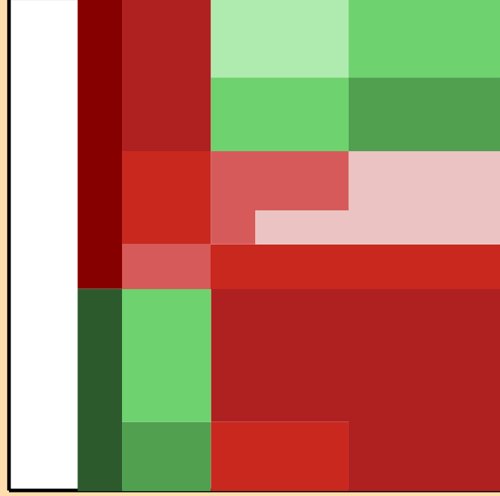
\Delta\sigma/\sigma vs. E for ^{144}\text{Ce}(n,p)
