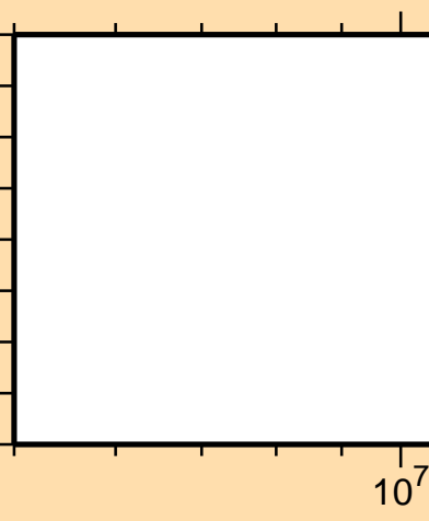
\sigma vs. E for ^{144}\text{Ce}(n,2n\alpha)
