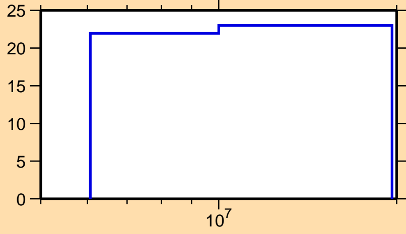
\Delta\sigma/\sigma vs. E for ^{144}\text{Ce}(n,2n)
