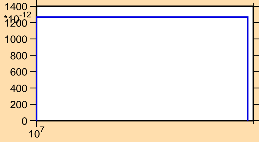
\sigma vs. E for ^{144}\text{Ce}(n,\text{nd})
