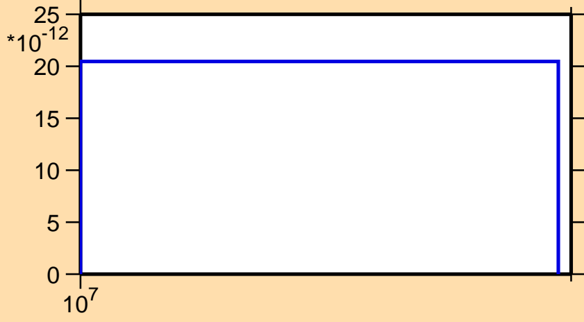
\sigma vs. E for ^{144}\text{Ce}(n,2np)
