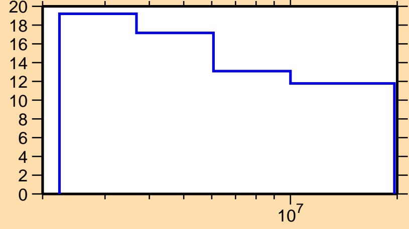
\Delta\sigma/\sigma vs. E for ^{144}\text{Ce}(n,n\text{onel.})
