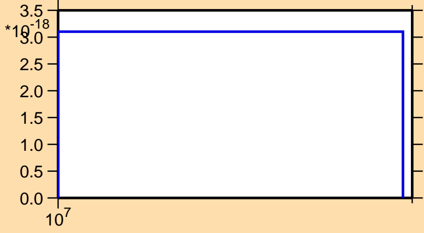
\sigma vs. E for ^{144}\text{Ce} (mt 11)
