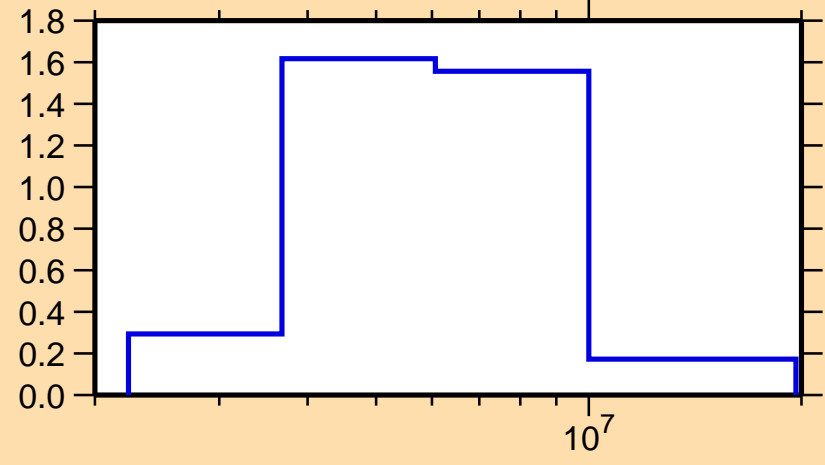
\sigma vs. E for ^{144}\text{Ce}(n,n\text{cont.})
