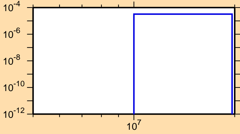
\sigma vs. E for ^{144}\text{Ce}(n,t)
