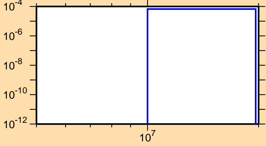
\sigma vs. E for ^{144}\text{Ce}(n,d)
