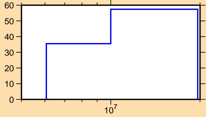
\Delta\sigma/\sigma vs. E for ^{144}\text{Ce}(n,ncont.)
