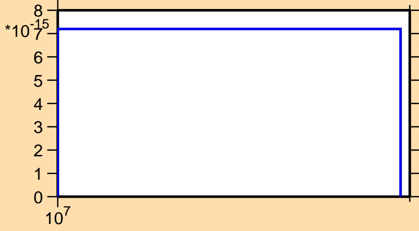
\sigma vs. E for ^{144}\text{Ce}(n,\text{He}3)
