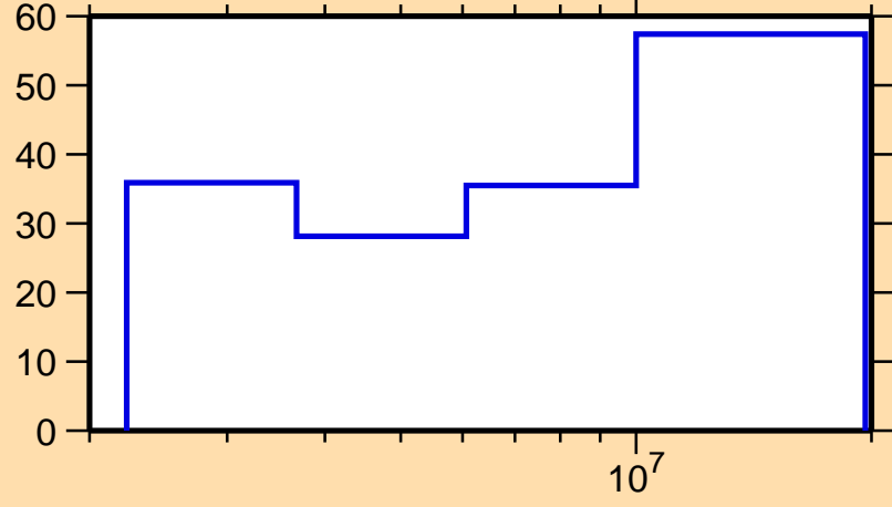
\Delta\sigma/\sigma vs. E for ^{144}\text{Ce}(n,n\text{cont.})
