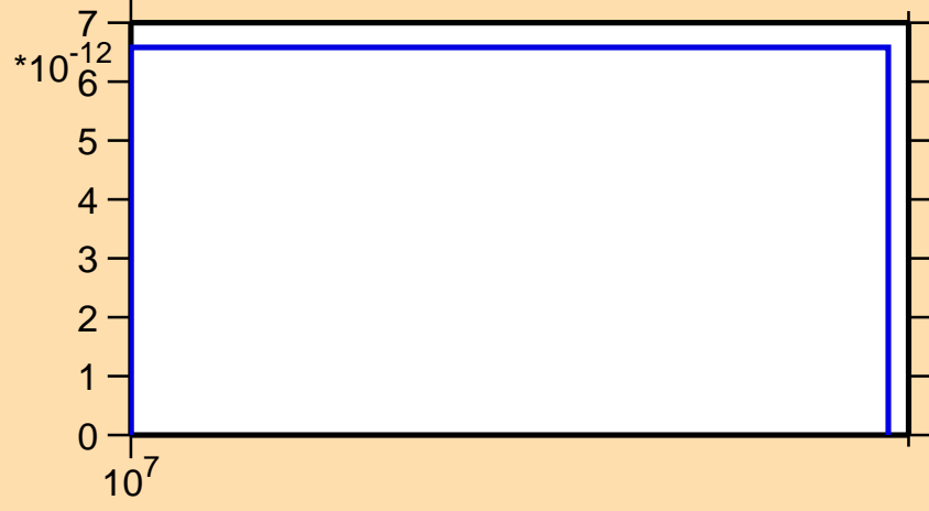
\sigma vs. E for ^{144}\text{Ce}(n,3n\alpha)
