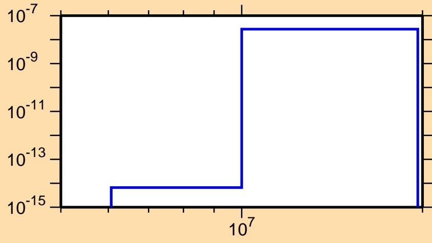
\sigma vs. E for ^{144}\text{Ce}(n,2n\alpha)
