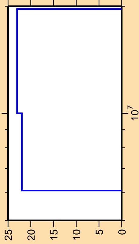
\Delta\sigma/\sigma vs. E for ^{144}\text{Ce}(n,2n)
