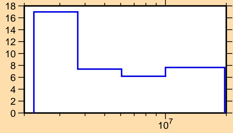
\Delta\sigma/\sigma vs. E for ^{144}\text{Ce}(n,\text{tot.})
