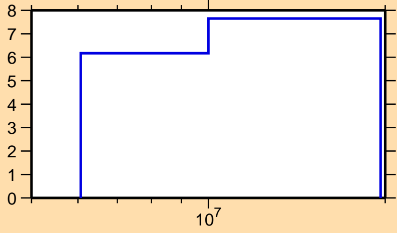
\Delta\sigma/\sigma vs. E for ^{144}\text{Ce}(n,\text{tot.})
