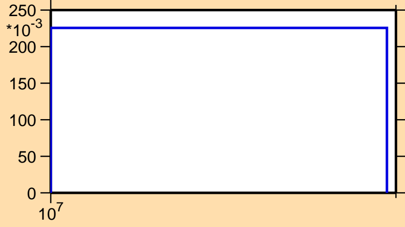
\sigma vs. E for ^{144}\text{Ce}(n,3n)
