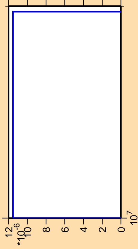
\Delta\sigma/\sigma vs. E for ^{144}\text{Ce} (mt 11)
