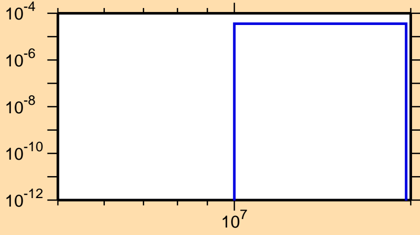
\sigma vs. E for ^{144}\text{Ce}(n,np)
