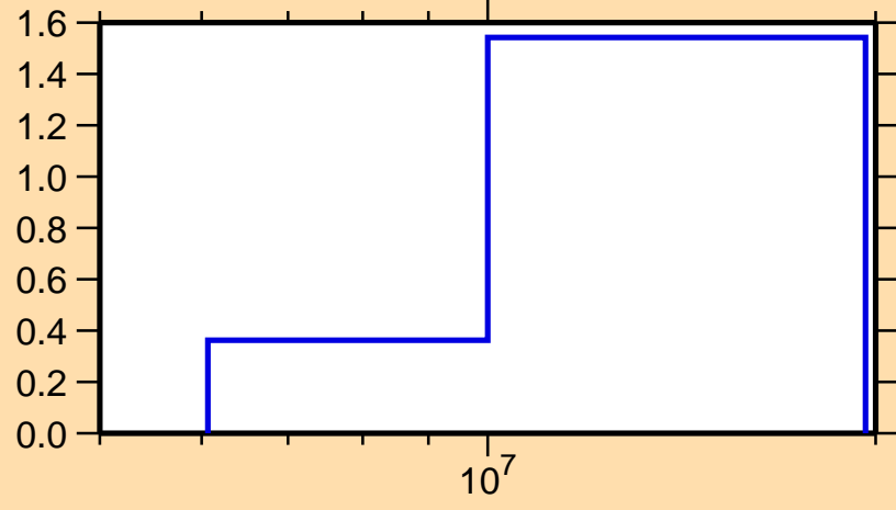
\sigma vs. E for ^{144}\text{Ce}(n,2n)
