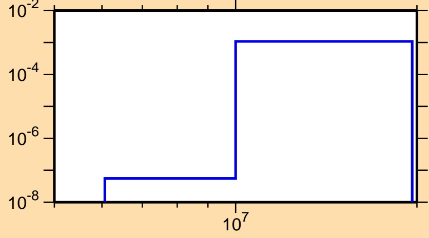
\sigma vs. E for ^{144}\text{Ce}(n,p)
