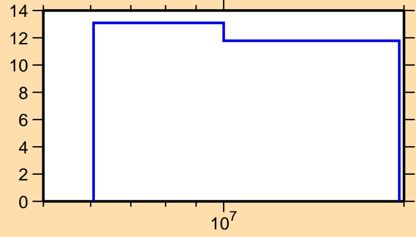
\Delta\sigma/\sigma vs. E for ^{144}\text{Ce}(n,\text{nonel.})
