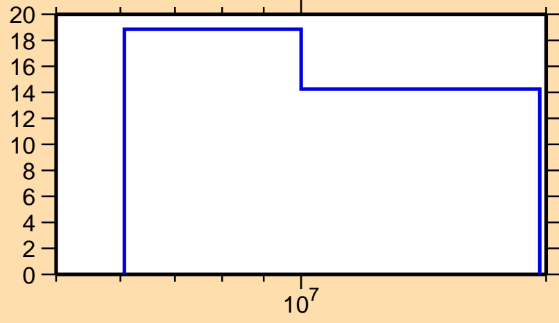
\Delta\sigma/\sigma vs. E for ^{144}\text{Ce}(n,\text{el.})
