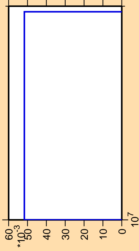
\Delta\sigma/\sigma vs. E for ^{144}\text{Ce}(n,\text{He}3)
