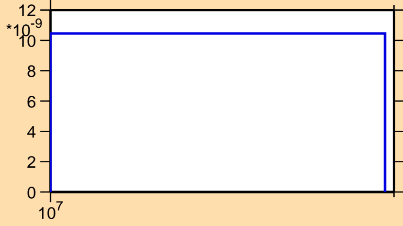
\sigma vs. E for ^{144}\text{Ce}(n,nt)
