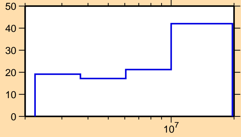
\Delta\sigma/\sigma vs. E for ^{144}\text{Ce}(n,\text{inel.})
