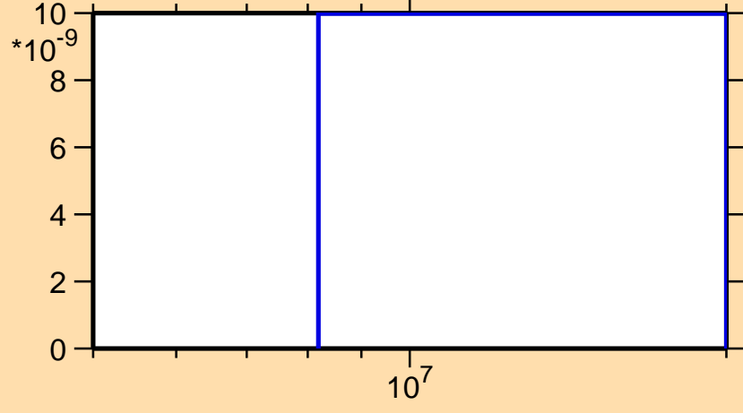
\sigma vs. E for ^{144}\text{Ce}(n,\text{nt})
