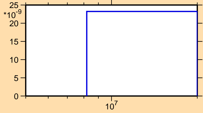
\sigma vs. E for ^{144}\text{Ce}(n,2n\alpha)
