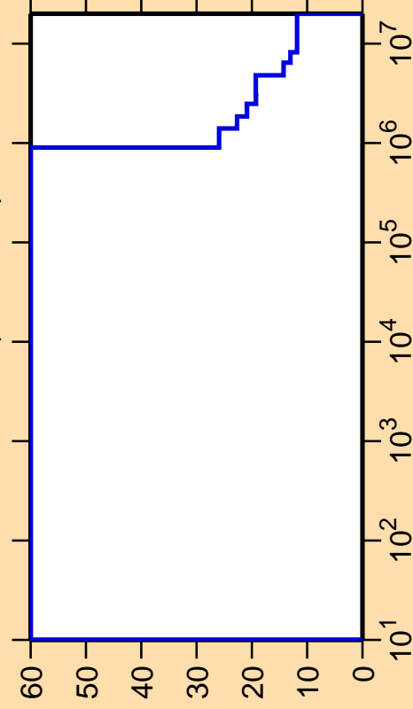
\Delta\sigma/\sigma vs. E for ^{144}\text{Ce}(n,\text{nonel.})
