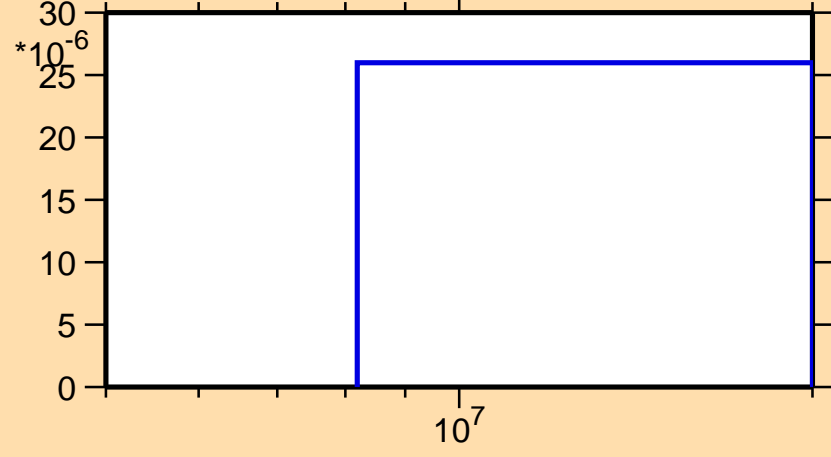
\sigma vs. E for ^{144}\text{Ce}(n,t)
