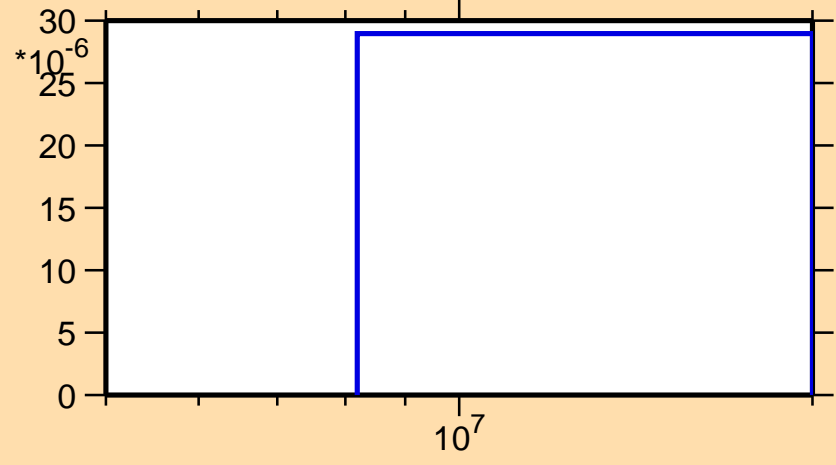
\sigma vs. E for ^{144}\text{Ce}(n,np)
