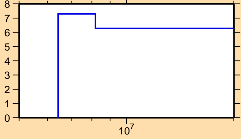
\Delta\sigma/\sigma vs. E for ^{144}\text{Ce}(n,\text{tot.})
