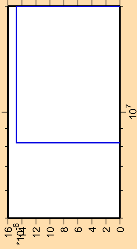
\Delta\sigma/\sigma vs. E for ^{144}\text{Ce}(\text{mt } 11)
