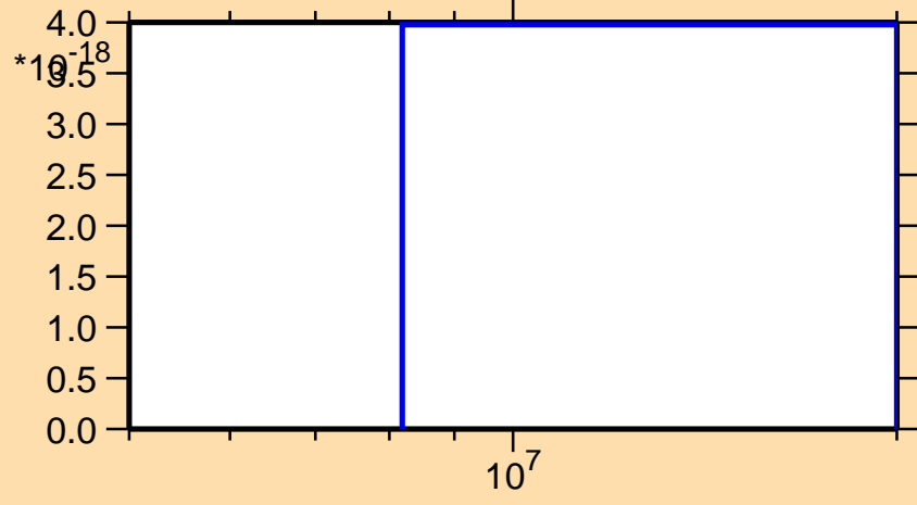
\sigma vs. E for ^{144}\text{Ce}(\text{mt } 11)
