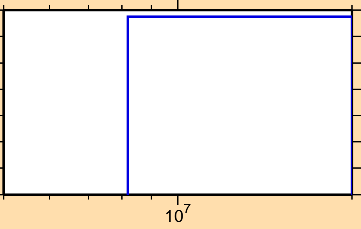
\sigma vs. E for ^{144}\text{Ce}(n,\text{nd})
