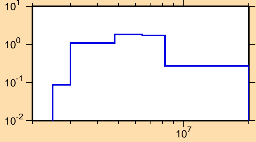
\sigma vs. E for ^{144}\text{Ce}(n,n\text{cont.})
