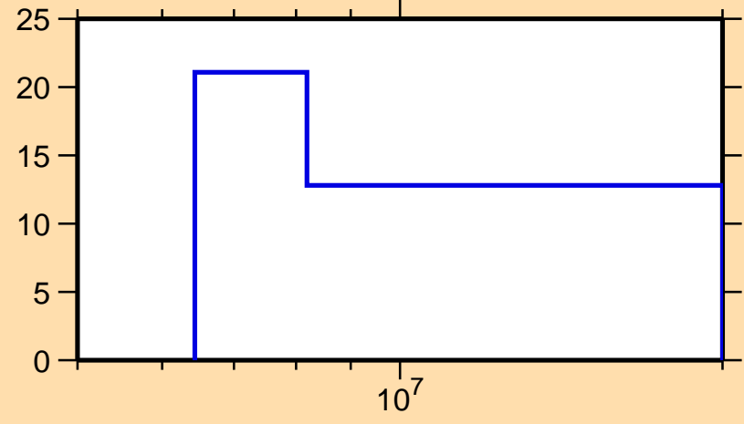
\Delta\sigma/\sigma vs. E for ^{144}\text{Ce}(n,el.)
