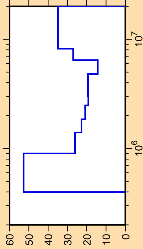
\Delta\sigma/\sigma vs. E for ^{144}\text{Ce}(n,\text{inel.})
