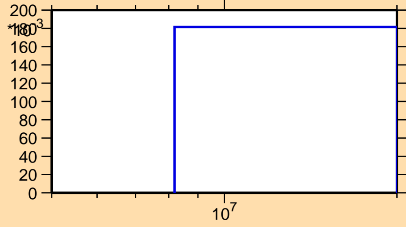
\sigma vs. E for ^{144}\text{Ce}(n,3n)
