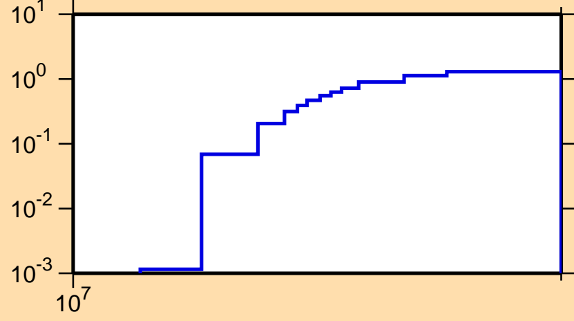
\sigma vs. E for ^{145}\text{Ce}(n,3n)
