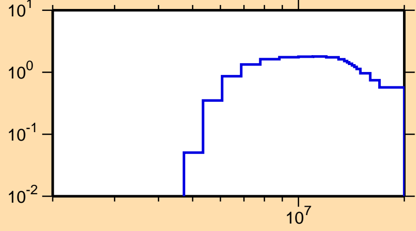
\sigma vs. E for ^{145}\text{Ce}(n,2n)
