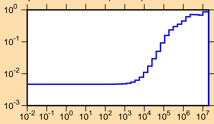
\mu vs. E for ^{145}\text{Ce}(\text{mt251})
