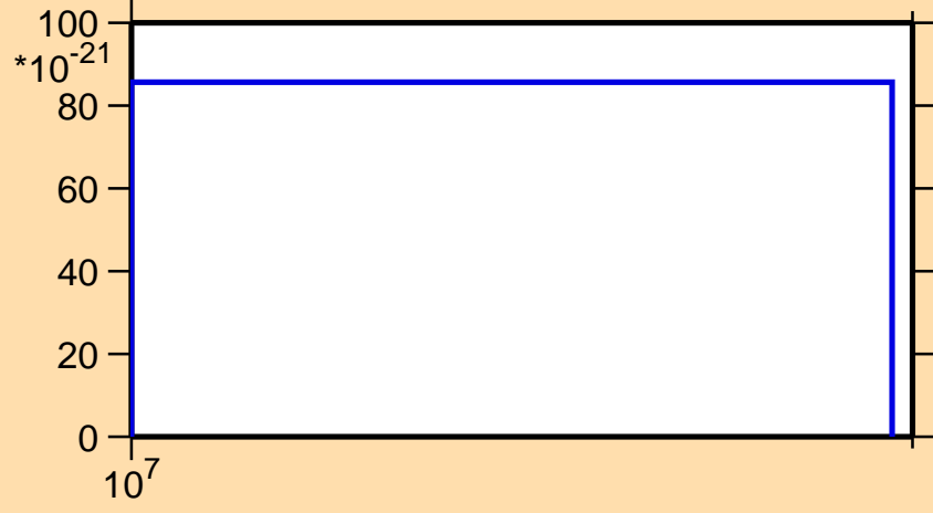
\sigma vs. E for ^{145}\text{Ce} (mt 11)
