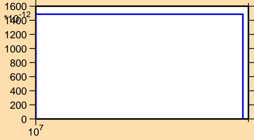
\sigma vs. E for ^{145}\text{Ce}(n,2np)
