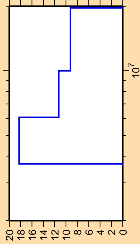
\Delta\sigma/\sigma vs. E for ^{145}\text{Ce}(n,2n)
