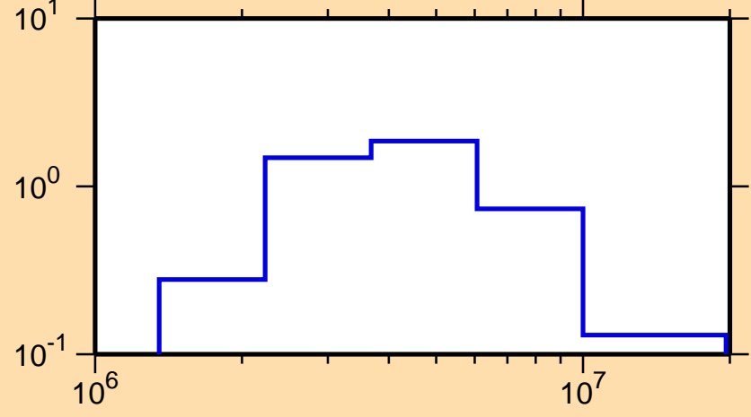
\sigma vs. E for ^{145}\text{Ce}(n,n\text{cont.})
