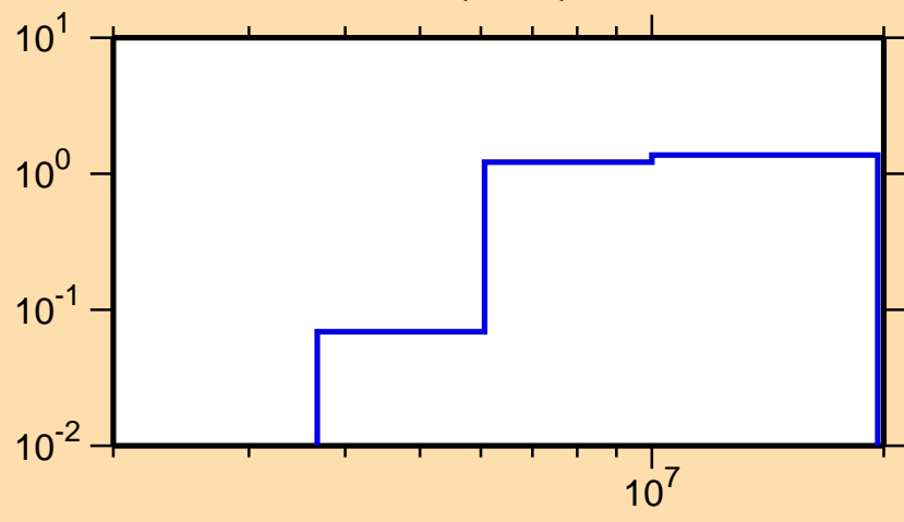
\sigma vs. E for ^{145}\text{Ce}(n,2n)
