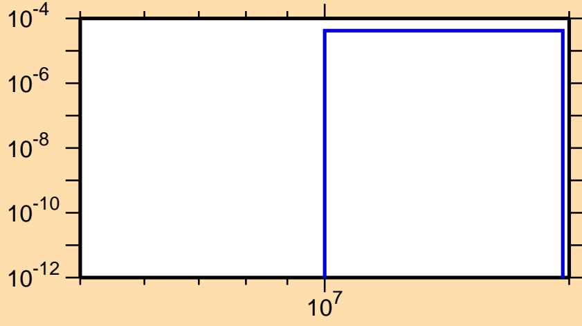
\sigma vs. E for ^{145}\text{Ce}(n,np)
