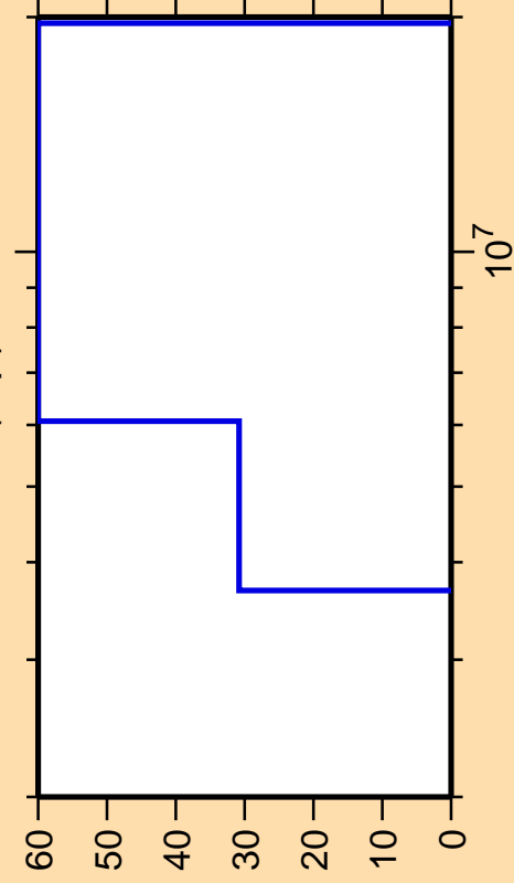
\Delta\sigma/\sigma vs. E for ^{145}\text{Ce}(n,p)
