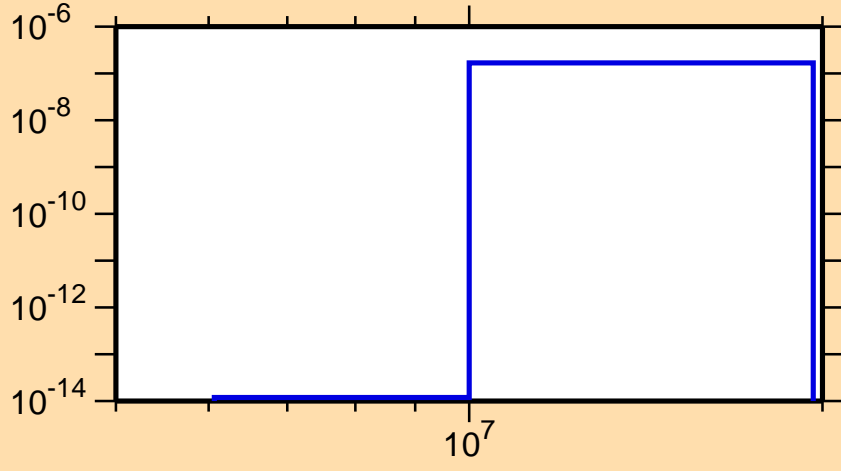
\sigma vs. E for ^{145}\text{Ce}(n,2n\alpha)
