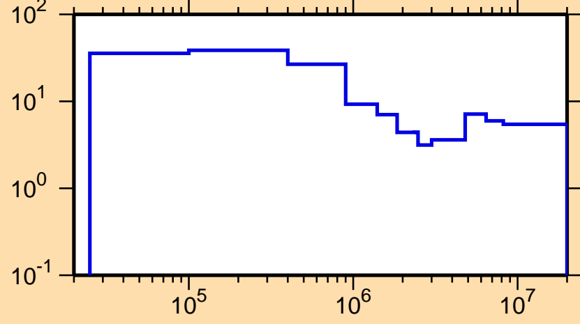
\Delta\sigma/\sigma vs. E for ^{145}\text{Ce}(n,\text{nonel.})
