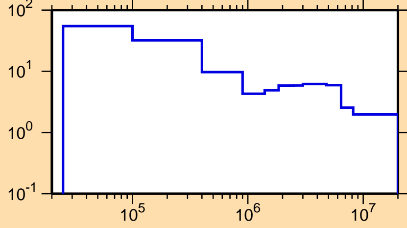
\Delta\sigma/\sigma vs. E for ^{145}\text{Ce}(n,\text{tot.})
