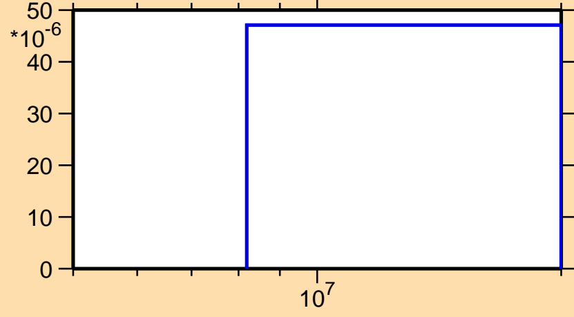
\sigma vs. E for ^{145}\text{Ce}(n,t)
