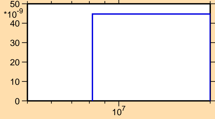
\sigma vs. E for ^{145}\text{Ce}(n,\text{nd})
