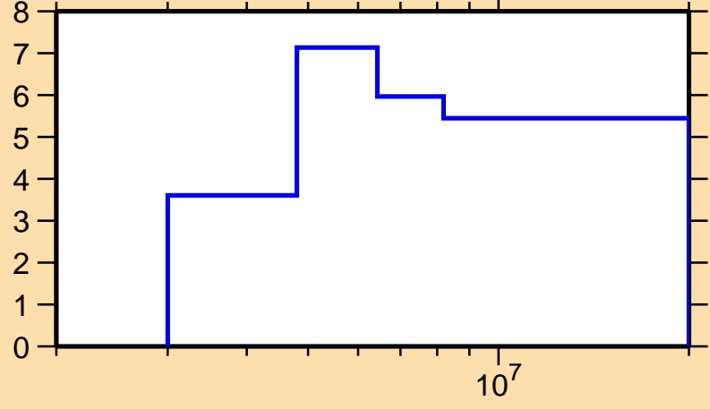
\Delta\sigma/\sigma vs. E for ^{145}\text{Ce}(n,\text{nonel.})
