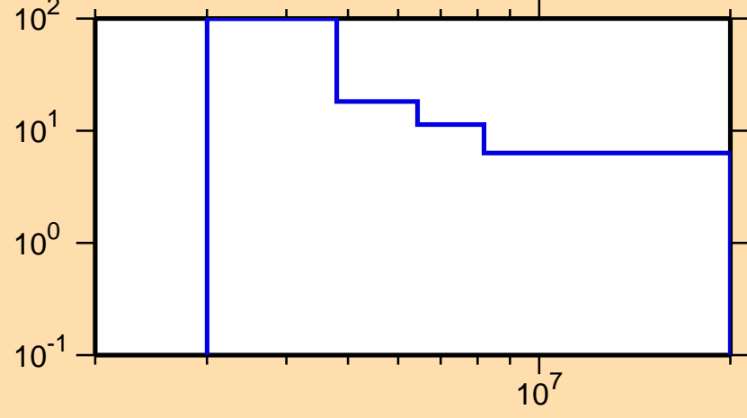
\Delta\sigma/\sigma vs. E for ^{145}\text{Ce}(n,2n)
