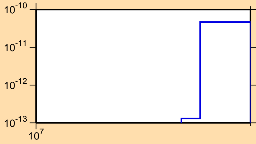
\sigma vs. E for ^{146}\text{Ce}(n,3n\alpha)
