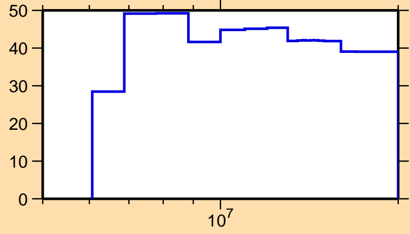
\Delta\sigma/\sigma vs. E for ^{146}\text{Ce}(n,ncont.)
