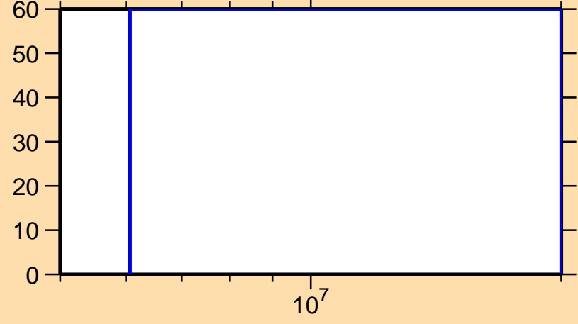
\Delta\sigma/\sigma vs. E for ^{146}\text{Ce}(n,\gamma)
