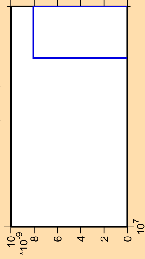
\Delta\sigma/\sigma vs. E for ^{146}\text{Ce} (mt 11)
