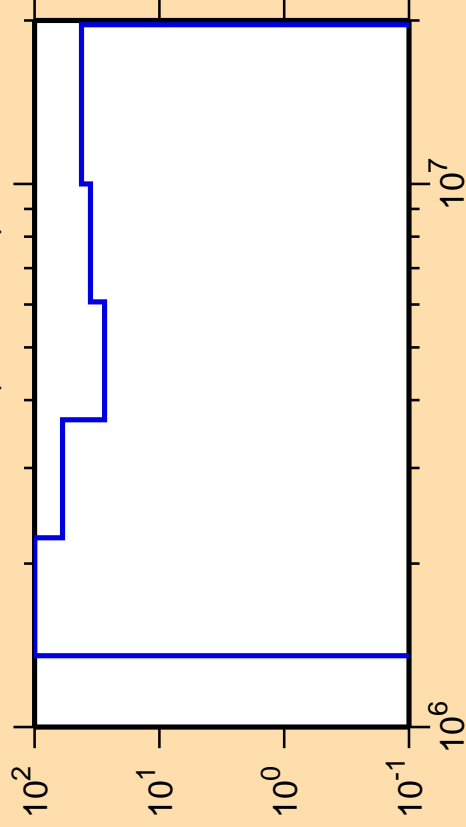
\Delta\sigma/\sigma vs. E for ^{146}\text{Ce}(n,\text{ncont.})
