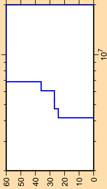
\Delta\sigma/\sigma vs. E for ^{147}\text{Ce}(n,n\text{cont.})
