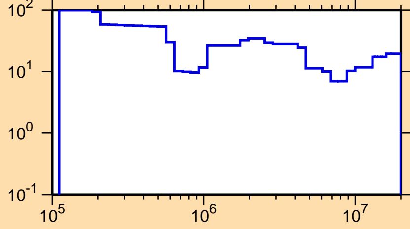
\Delta\sigma/\sigma vs. E for ^{147}\text{Ce}(n,\text{tot.})
