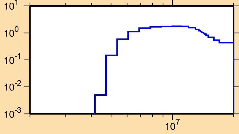
\sigma vs. E for ^{147}\text{Ce}(n,2n)
