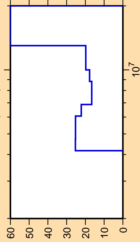
\Delta\sigma/\sigma vs. E for ^{147}\text{Ce}(n,2n)
