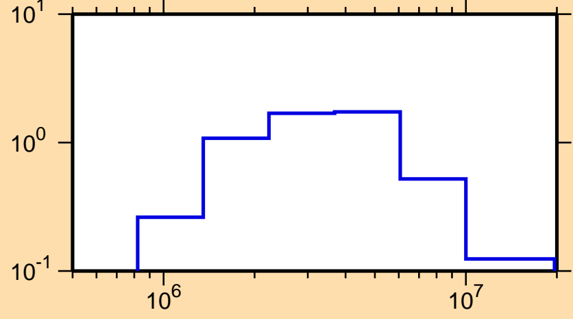
\sigma vs. E for ^{147}\text{Ce}(n,n\text{cont.})
