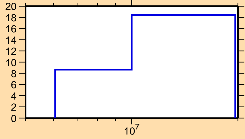
\Delta\sigma/\sigma vs. E for ^{147}\text{Ce}(n,el.)
