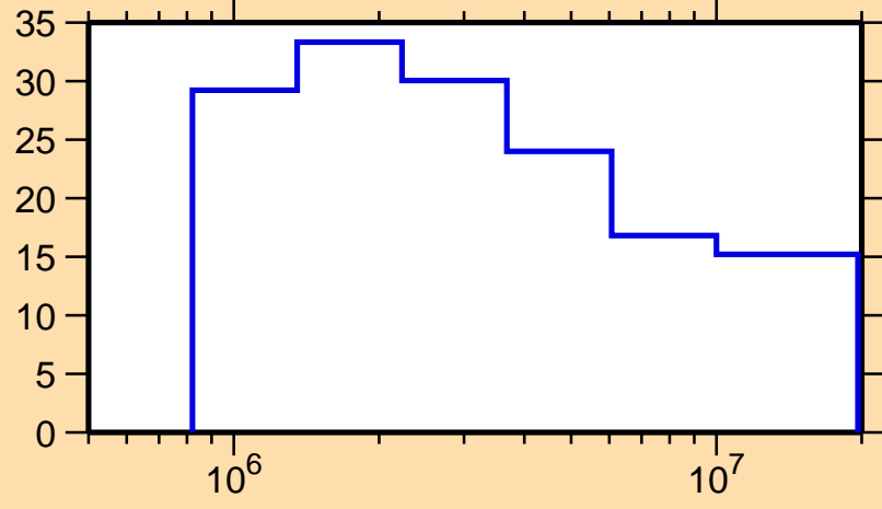
\Delta\sigma/\sigma vs. E for ^{147}\text{Ce}(n,n\text{onel.})
