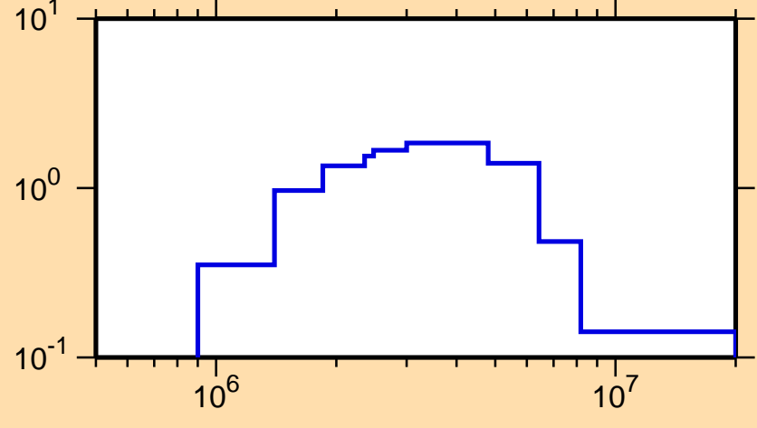
\sigma vs. E for ^{147}\text{Ce}(n,n\text{cont.})
