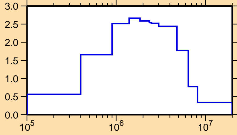
\sigma vs. E for ^{147}\text{Ce}(n,\text{inel.})
