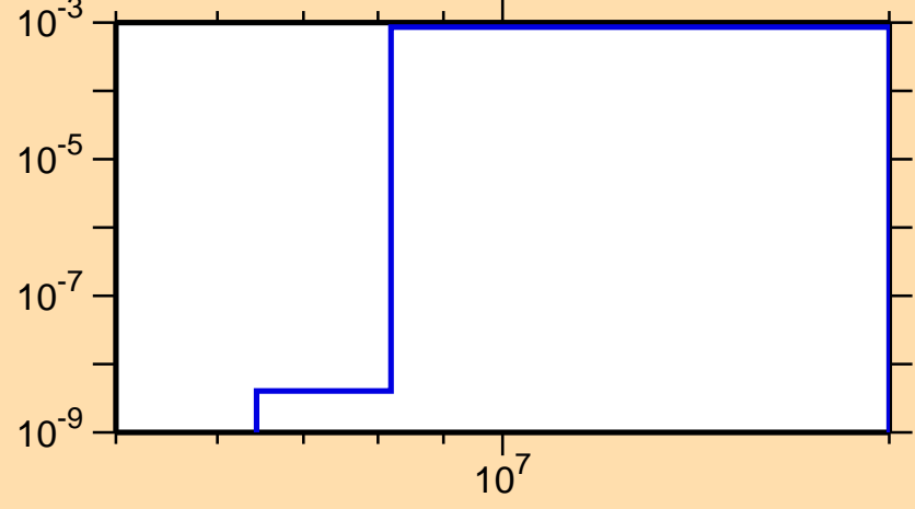
\sigma vs. E for ^{147}\text{Ce}(n,p)
