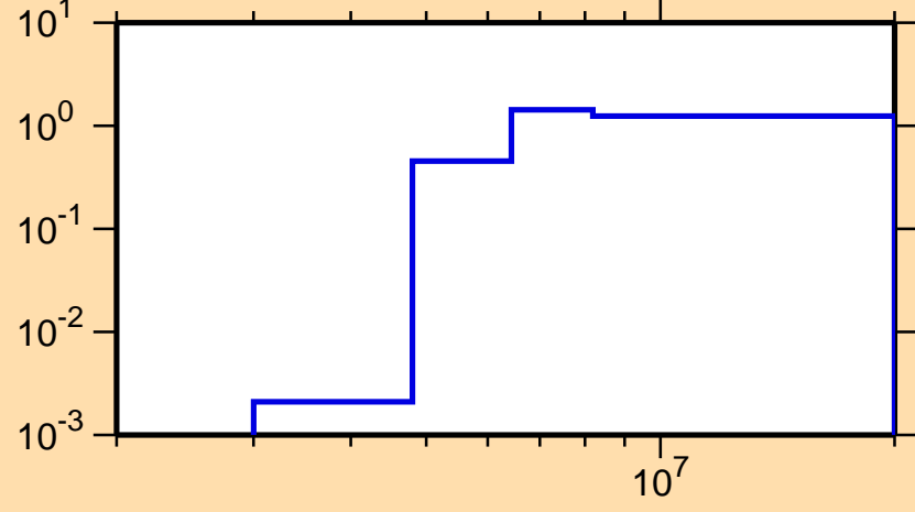
\sigma vs. E for ^{147}\text{Ce}(n,2n)
