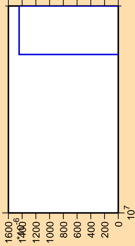
\Delta\sigma/\sigma vs. E for ^{148}\text{Ce} (mt 11)
