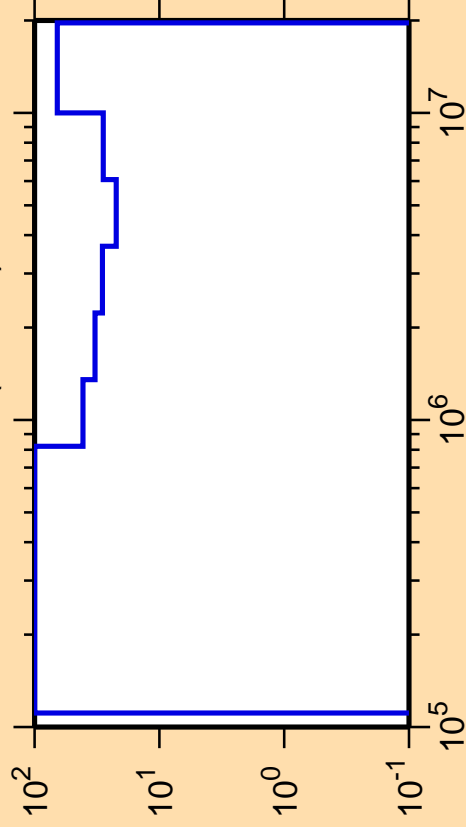
\Delta\sigma/\sigma vs. E for ^{148}\text{Ce}(n,\text{inel.})
