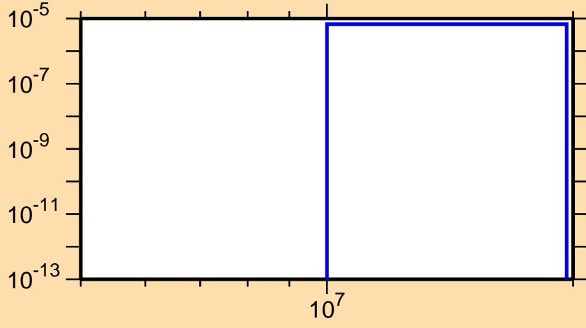
\sigma vs. E for ^{148}\text{Ce}(n,t)
