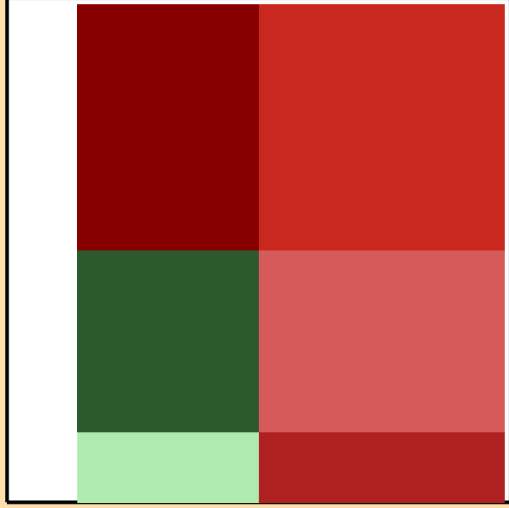
\Delta\sigma/\sigma vs. E for ^{148}\text{Ce}(n,p)
