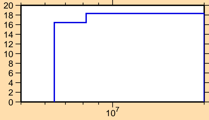
\Delta\sigma/\sigma vs. E for ^{148}\text{Ce}(n,\text{nonel.})
