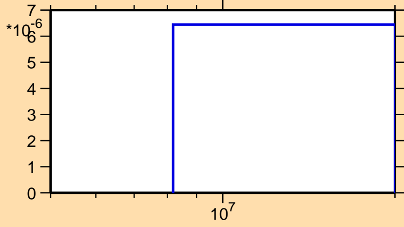
\sigma vs. E for ^{148}\text{Ce}(n,d)
