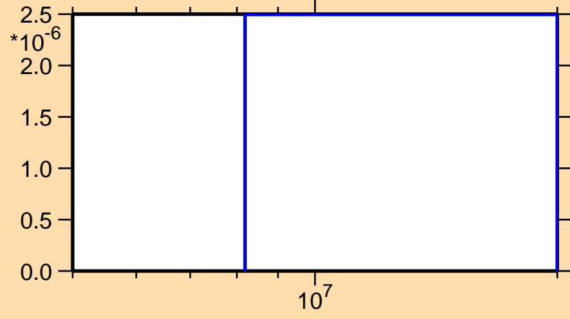
\sigma vs. E for ^{148}\text{Ce}(n,np)
