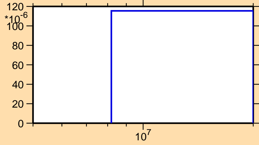
\sigma vs. E for ^{148}\text{Ce}(n,p)
