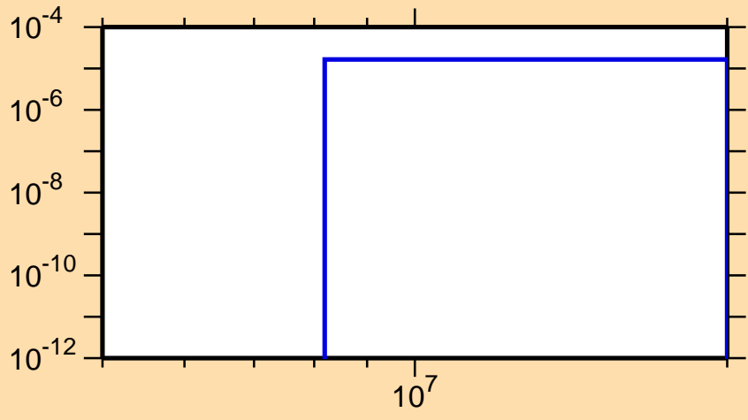
\sigma vs. E for ^{148}\text{Ce}(n,n\alpha)
