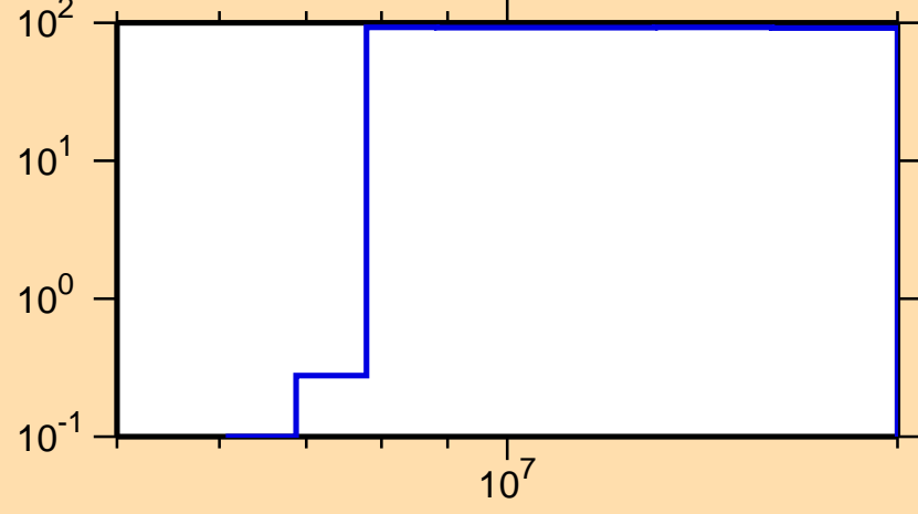
\Delta\sigma/\sigma vs. E for ^{149}\text{Ce}(n,p)
