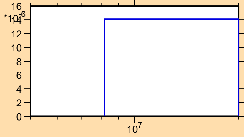
\sigma vs. E for ^{149}\text{Ce}(n,\alpha)
