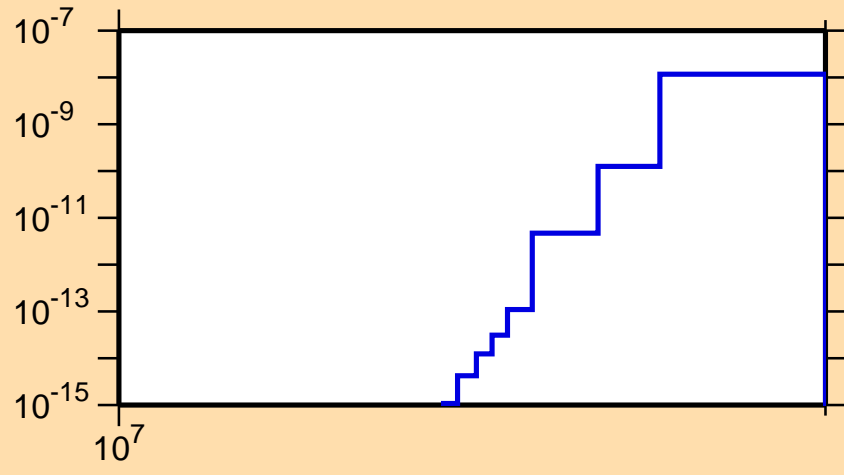
\sigma vs. E for ^{150}\text{Ce}(n,2n\alpha)
