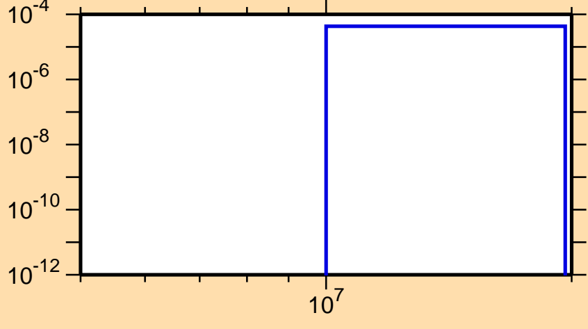
\sigma vs. E for ^{150}\text{Ce}(n,p)
