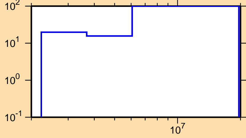
\Delta\sigma/\sigma vs. E for ^{150}\text{Ce}(n,\text{inel.})
