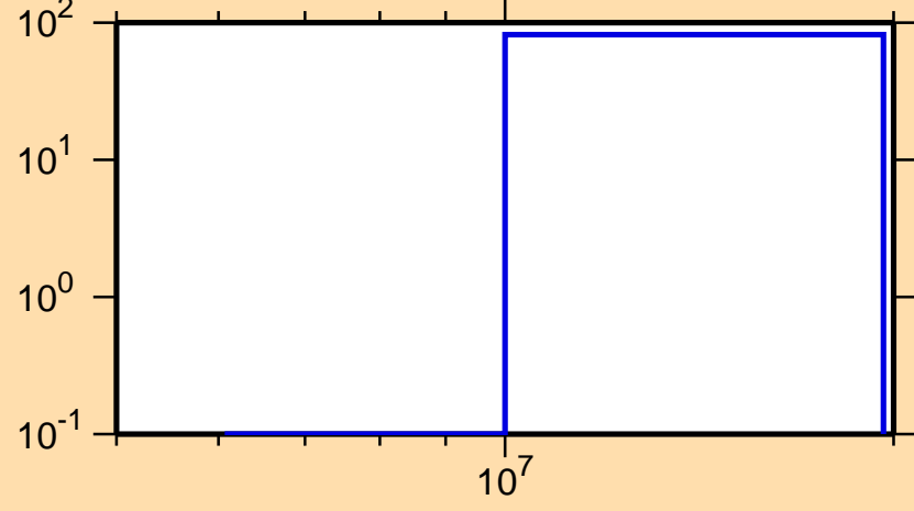
\Delta\sigma/\sigma vs. E for ^{150}\text{Ce}(n,p)
