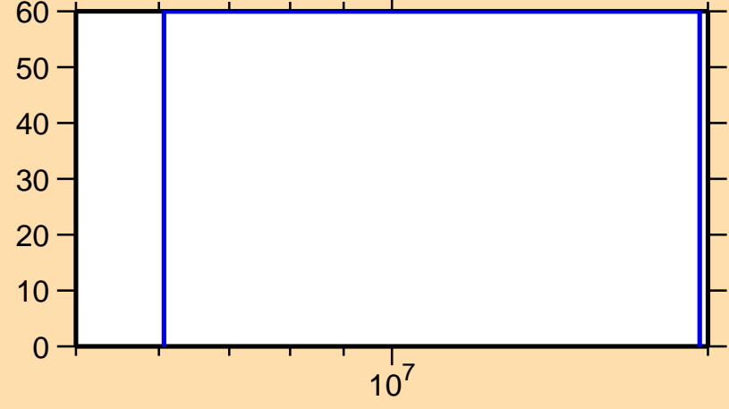
\Delta\sigma/\sigma vs. E for ^{150}\text{Ce}(n,ncont.)
