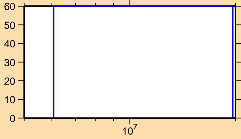
\Delta\sigma/\sigma vs. E for ^{150}\text{Ce}(n,n\text{cont.})
