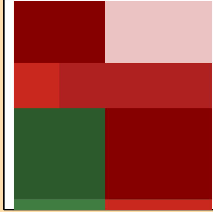
\Delta\sigma/\sigma vs. E for ^{150}\text{Ce}(n,n\text{cont.})
