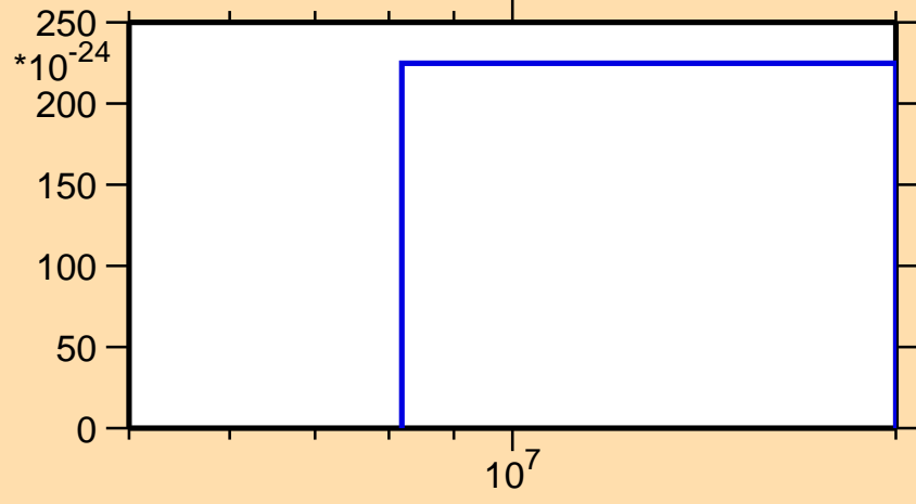
\sigma vs. E for ^{150}\text{Ce}(\text{mt } 11)
