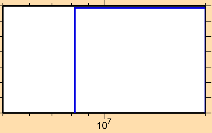
\sigma vs. E for ^{150}\text{Ce}(n,d)
