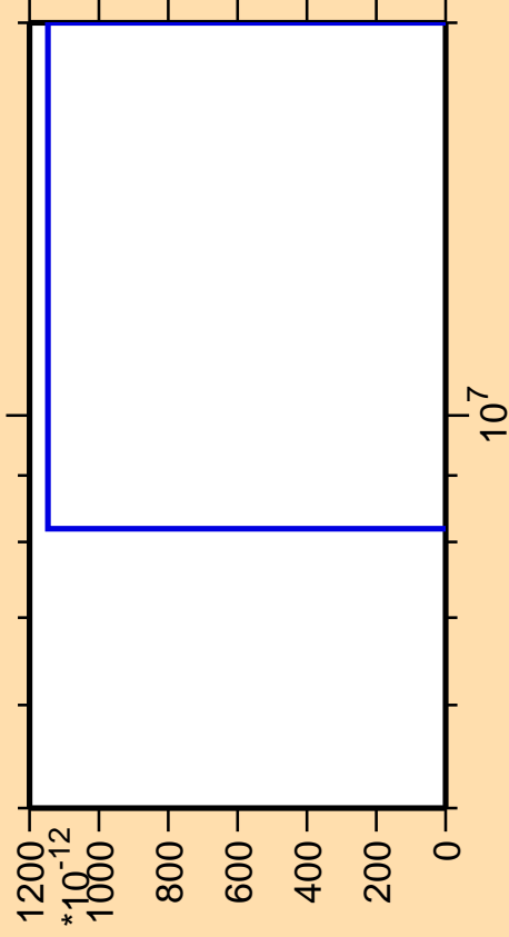
\Delta\sigma/\sigma vs. E for ^{150}\text{Ce}(\text{mt } 11)
