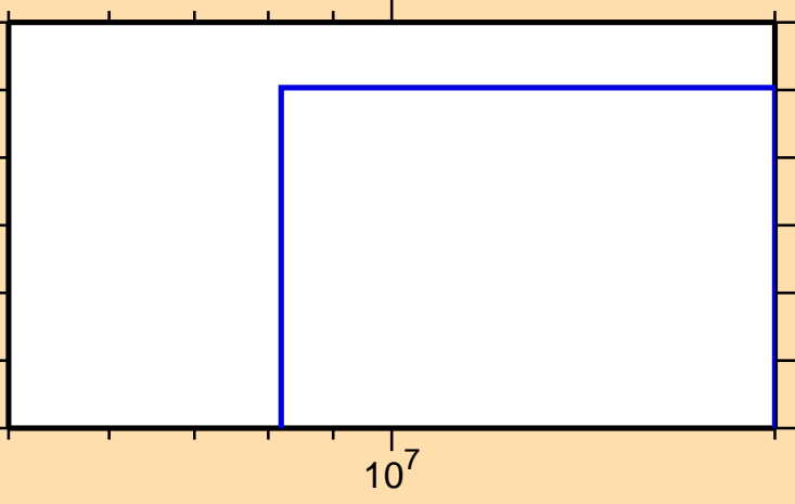
\sigma vs. E for ^{150}\text{Ce}(n,2n\alpha)
