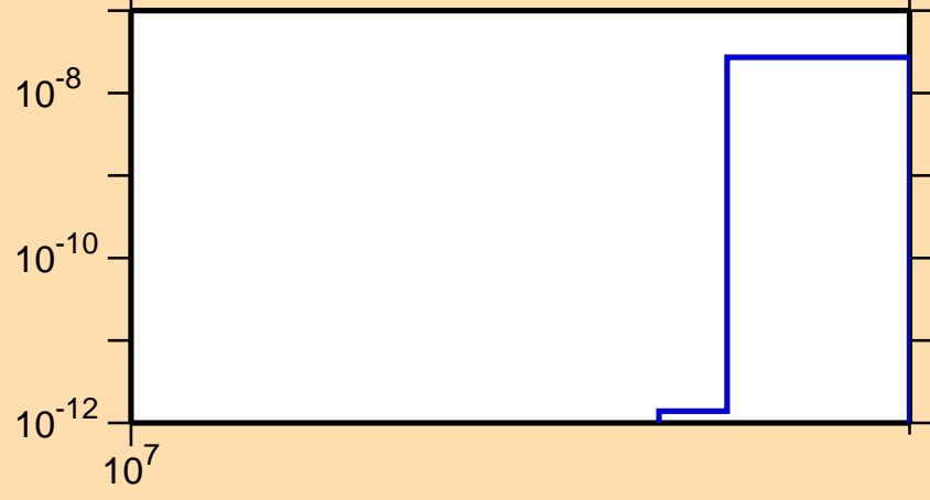
\sigma vs. E for ^{151}\text{Ce}(n,\text{nd})
