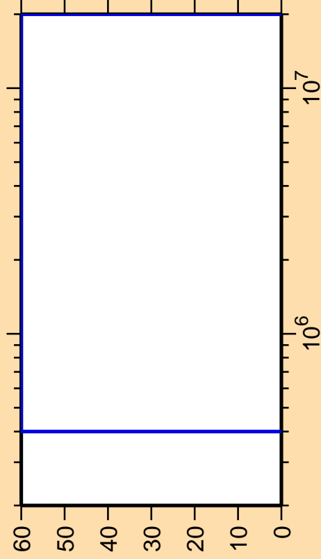
\Delta\sigma/\sigma vs. E for ^{151}\text{Ce}(n,\gamma)
