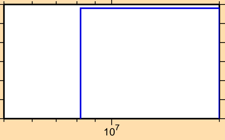
\sigma vs. E for ^{151}\text{Ce}(n,nt)
