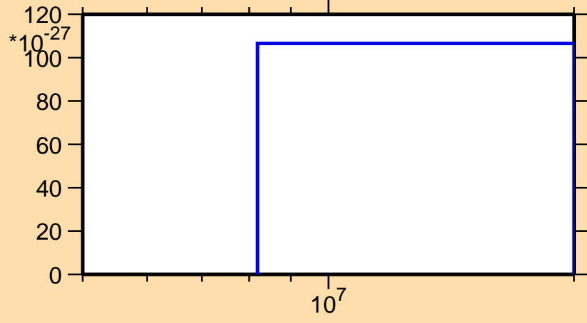
\sigma vs. E for ^{151}\text{Ce}(\text{mt } 11)
