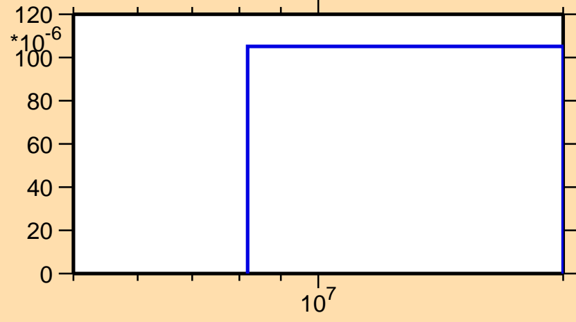
\sigma vs. E for ^{151}\text{Ce}(n,p)
