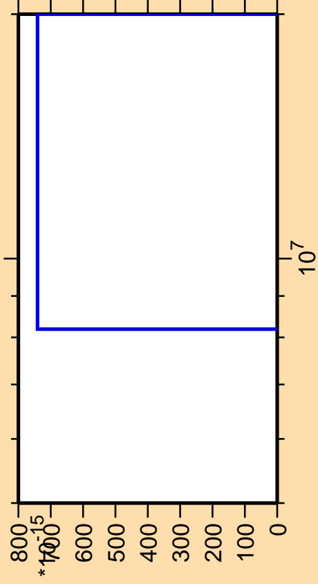
\Delta\sigma/\sigma vs. E for ^{151}\text{Ce}(\text{mt } 11)
