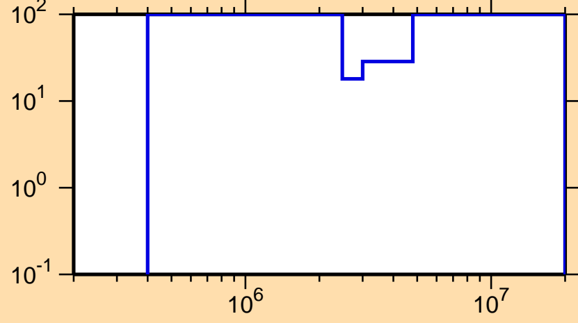
\Delta\sigma/\sigma vs. E for ^{151}\text{Ce}(n,n\text{cont.})
