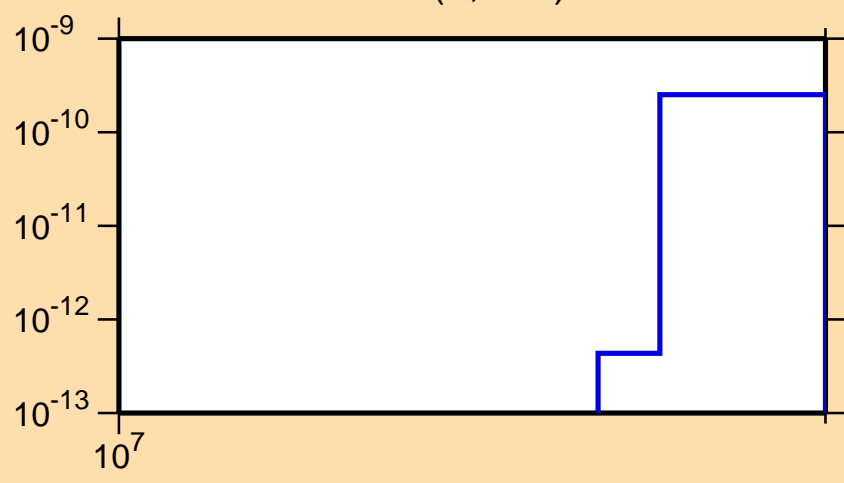
\sigma vs. E for ^{152}\text{Ce}(n,2n\alpha)
