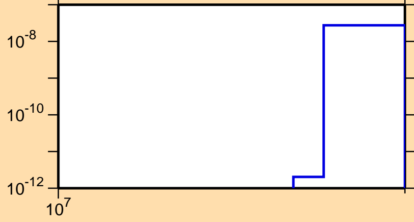
\sigma vs. E for ^{152}\text{Ce}(n,nt)
