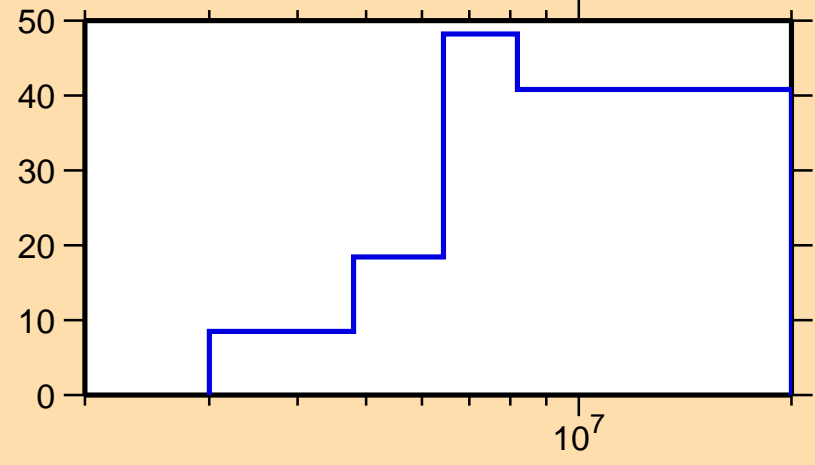
\Delta\sigma/\sigma vs. E for ^{152}\text{Ce}(n,\text{inel.})
