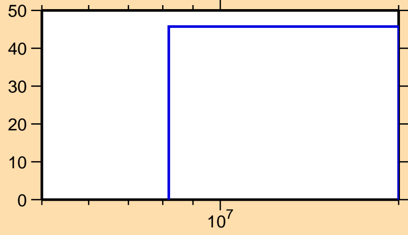
\Delta\sigma/\sigma vs. E for ^{152}\text{Ce}(n,n\text{cont.})
