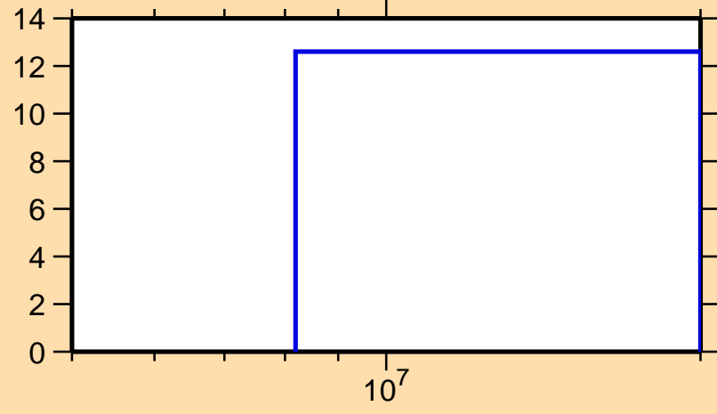
\Delta\sigma/\sigma vs. E for ^{152}\text{Ce}(n,\text{nonel.})
