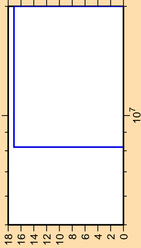
\Delta\sigma/\sigma vs. E for ^{152}\text{Ce}(n,3n)
