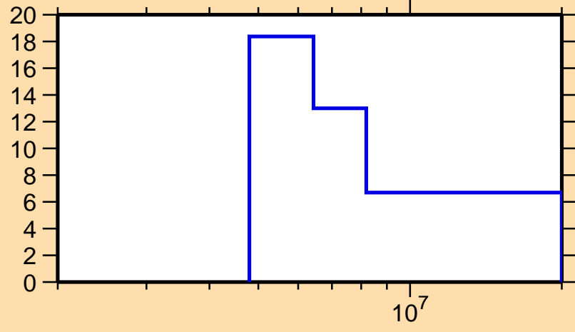
\Delta\sigma/\sigma vs. E for ^{152}\text{Ce}(n,\text{el.})
