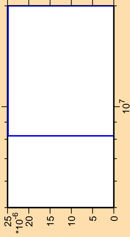
\Delta\sigma/\sigma vs. E for ^{152}\text{Ce}(n,2np)
