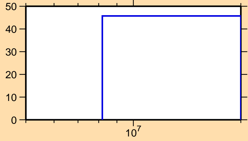
\Delta\sigma/\sigma vs. E for ^{152}\text{Ce}(n,ncont.)
