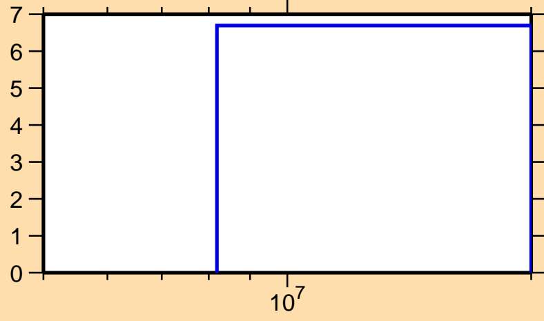
\Delta\sigma/\sigma vs. E for ^{152}\text{Ce}(n,\text{el.})
