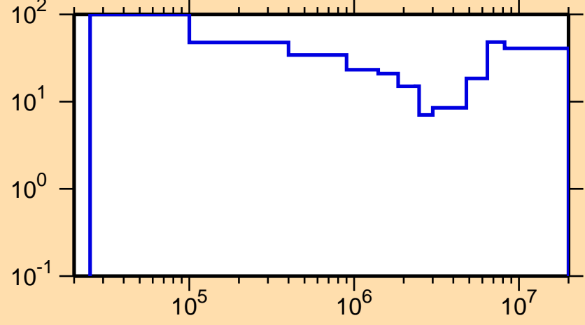
\Delta\sigma/\sigma vs. E for ^{152}\text{Ce}(n,\text{inel.})
