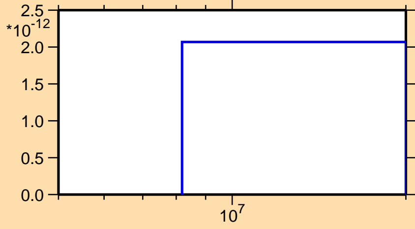
\sigma vs. E for ^{152}\text{Ce}(n,2n\alpha)
