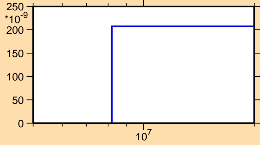
\sigma vs. E for ^{152}\text{Ce}(n,d)
