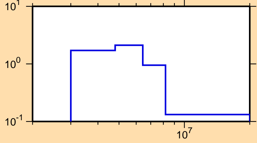
\sigma vs. E for ^{152}\text{Ce}(n,n\text{cont.})
