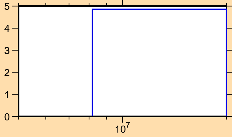
\Delta\sigma/\sigma vs. E for ^{152}\text{Ce}(n,\text{tot.})
