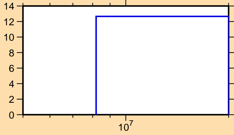
\Delta\sigma/\sigma vs. E for ^{152}\text{Ce}(n,2n)
