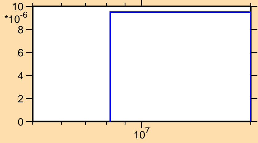
\sigma vs. E for ^{152}\text{Ce}(n,p)
