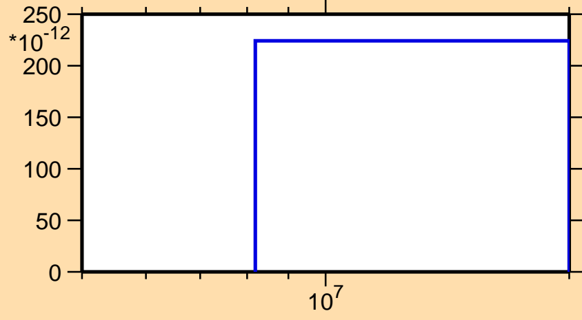
\sigma vs. E for ^{152}\text{Ce}(n,nt)
