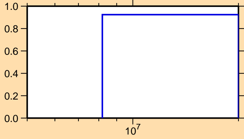
\sigma vs. E for ^{152}\text{Ce}(n,3n)
