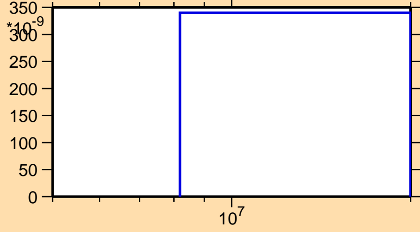
\sigma vs. E for ^{152}\text{Ce}(n,t)
