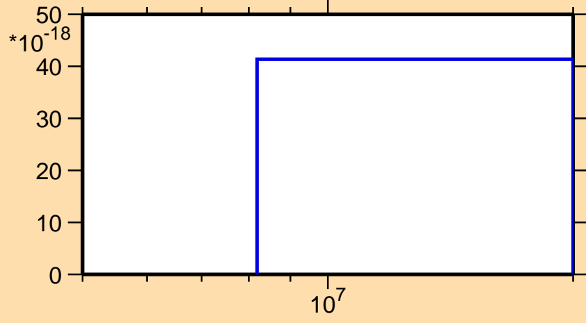
\sigma vs. E for ^{152}\text{Ce}(n,2np)
