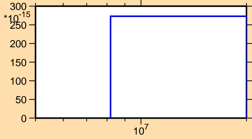
\sigma vs. E for ^{152}\text{Ce}(n,\text{nd})
