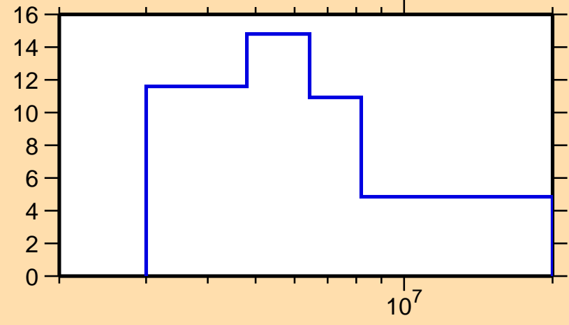
\Delta\sigma/\sigma vs. E for ^{152}\text{Ce}(n,\text{tot.})
