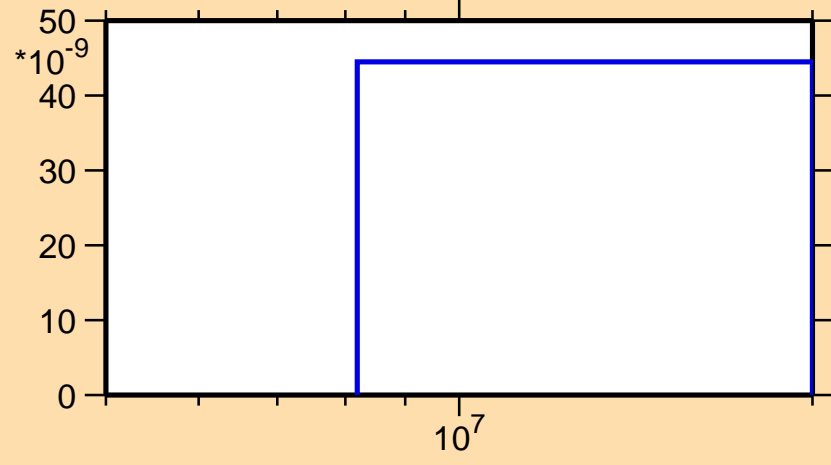
\sigma vs. E for ^{152}\text{Ce}(n,np)
