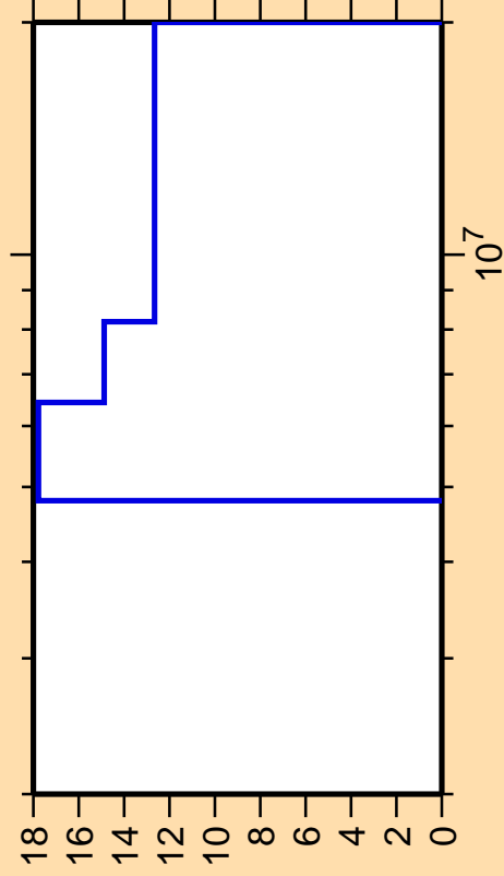
\Delta\sigma/\sigma vs. E for ^{152}\text{Ce}(n,2n)
