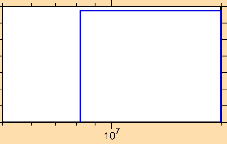
\sigma vs. E for ^{152}\text{Ce}(n,\alpha)
