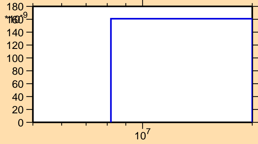
\sigma vs. E for ^{152}\text{Ce}(n,\alpha)
