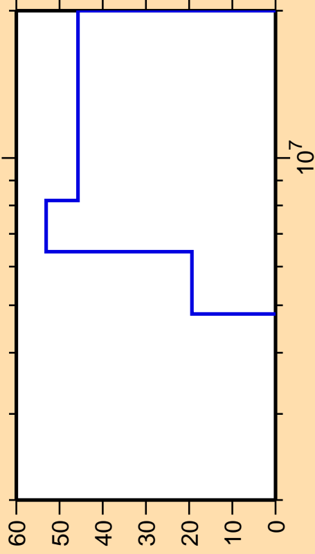
\Delta\sigma/\sigma vs. E for ^{152}\text{Ce}(n,n\text{cont.})
