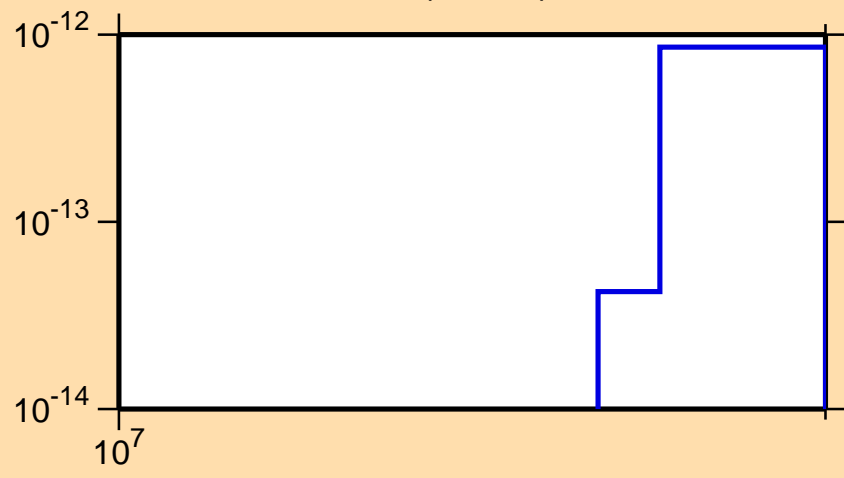
\sigma vs. E for ^{239}\text{Cf}(\text{mt } 34)
