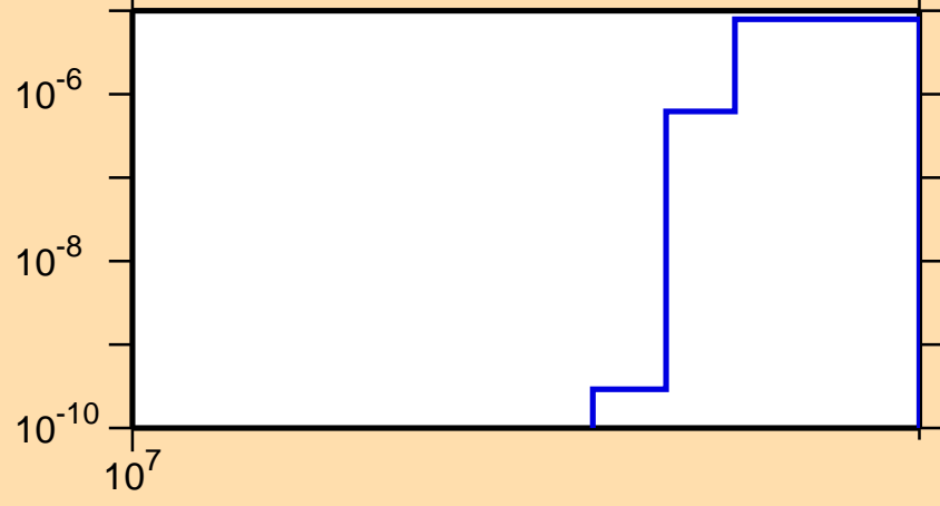
\sigma vs. E for ^{239}\text{Cf}(n,3n)
