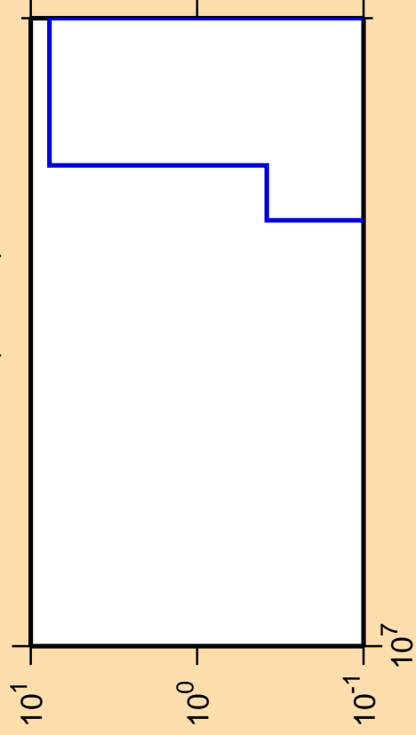
\Delta\sigma/\sigma vs. E for ^{239}\text{Cf}(\text{mt } 34)
