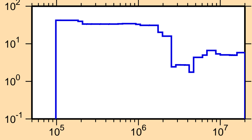
\Delta\sigma/\sigma vs. E for ^{239}\text{Cf}(n,\text{nonel.})
