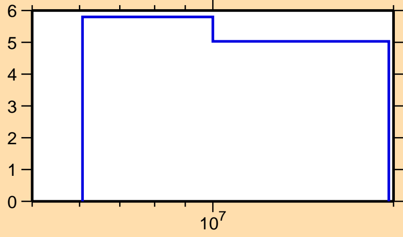
\Delta\sigma/\sigma vs. E for ^{239}\text{Cf}(n,\text{nonel.})
