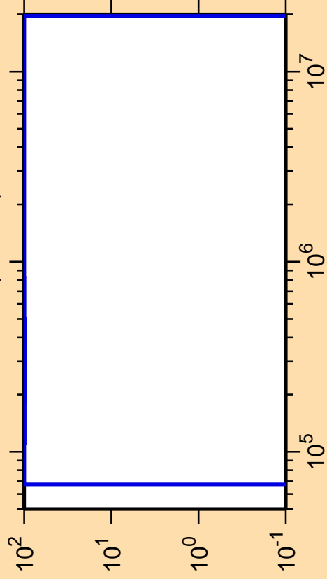
\Delta\sigma/\sigma vs. E for ^{239}\text{Cf}(n,\text{inel.})
