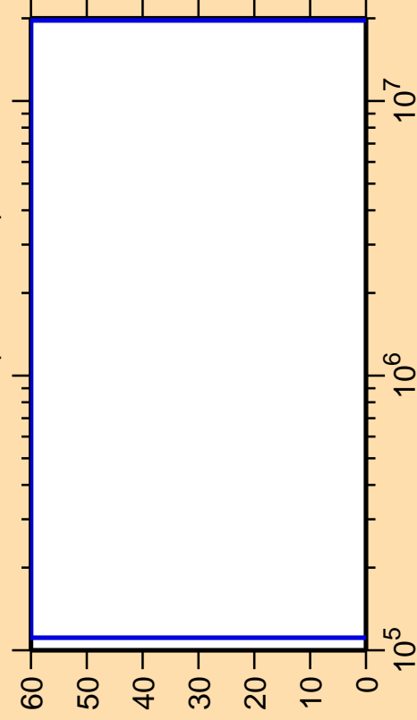
\Delta\sigma/\sigma vs. E for ^{239}\text{Cf}(n,\text{ncont.})
