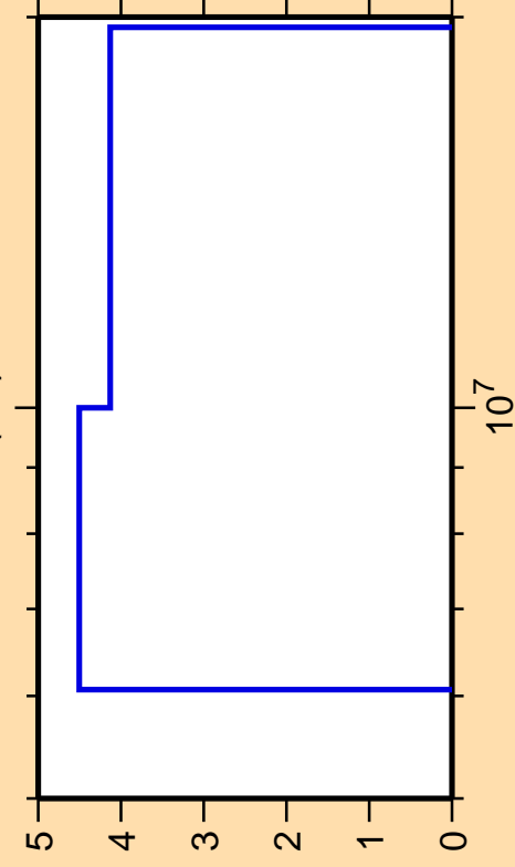
\Delta\sigma/\sigma vs. E for ^{239}\text{Cf}(n,f)
