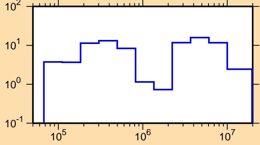
\Delta\sigma/\sigma vs. E for ^{239}\text{Cf}(n,\text{el.})
