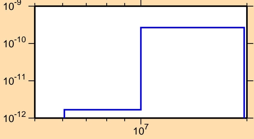
\sigma vs. E for ^{239}\text{Cf}(n,p\alpha)
