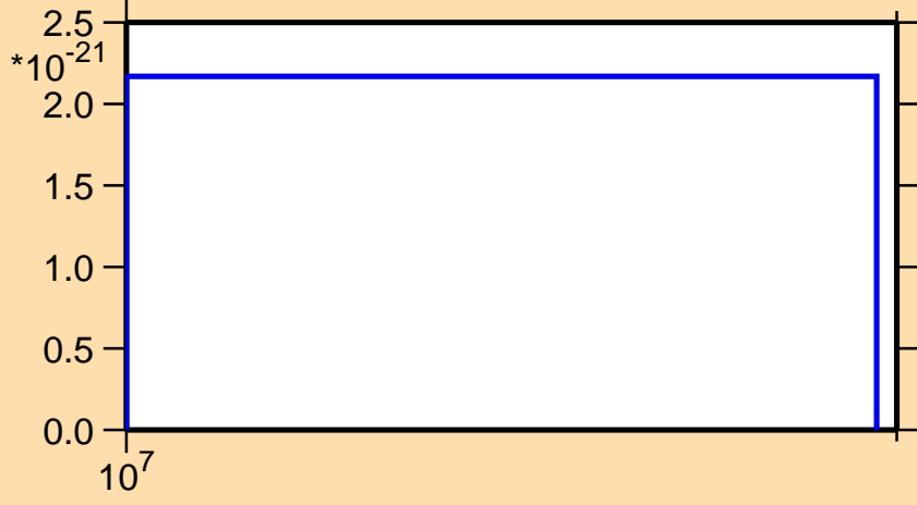
\sigma vs. E for ^{239}\text{Cf} (mt 42)
