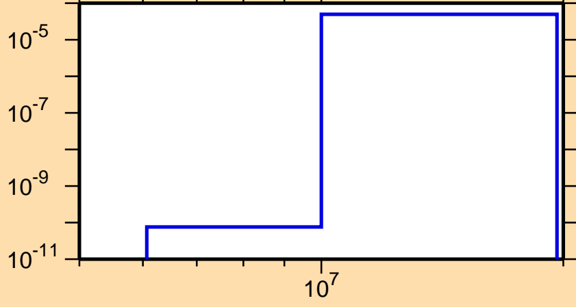
\sigma vs. E for ^{239}\text{Cf}(n,t)
