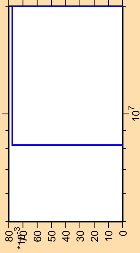
\Delta\sigma/\sigma vs. E for ^{239}\text{Cf} (mt 34)
