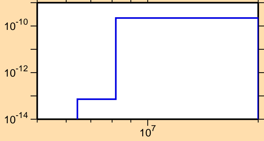
\sigma vs. E for ^{239}\text{Cf}(n,2n\alpha)
