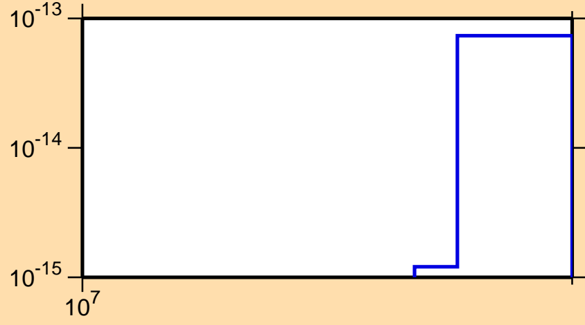
\sigma vs. E for ^{240}\text{Cf} (mt 34)
