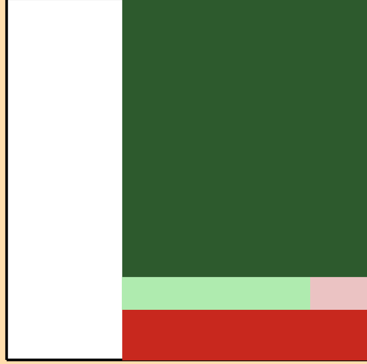
\Delta\sigma/\sigma vs. E for ^{240}\text{Cf}(n,2n)
