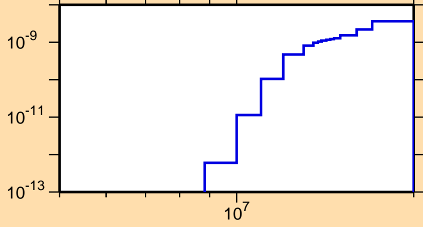
\sigma vs. E for ^{240}\text{Cf}(n,2n\alpha)
