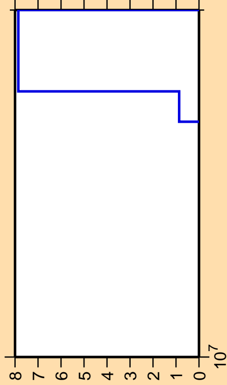
\Delta\sigma/\sigma vs. E for ^{240}\text{Cf}(n,3n\alpha)
