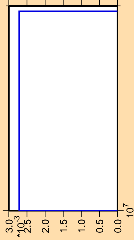
\Delta\sigma/\sigma vs. E for ^{240}\text{Cf} (mt 34)
