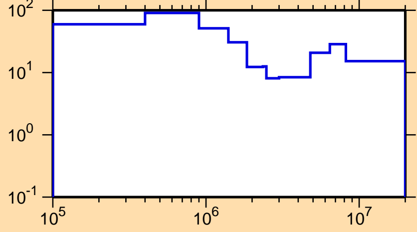
\Delta\sigma/\sigma vs. E for ^{240}\text{Cf}(n,\text{el.})
