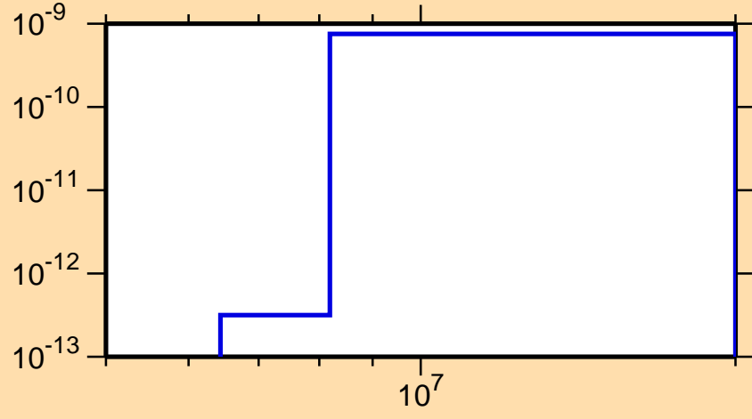
\sigma vs. E for ^{240}\text{Cf}(n,p\alpha)
