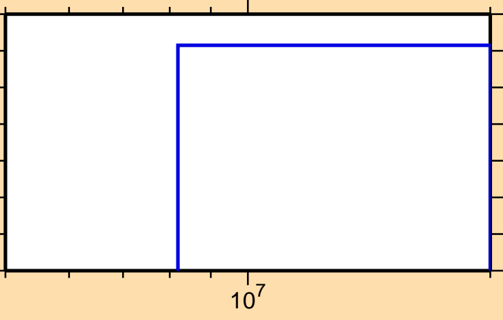
\sigma vs. E for ^{240}\text{Cf}(n,nd)
