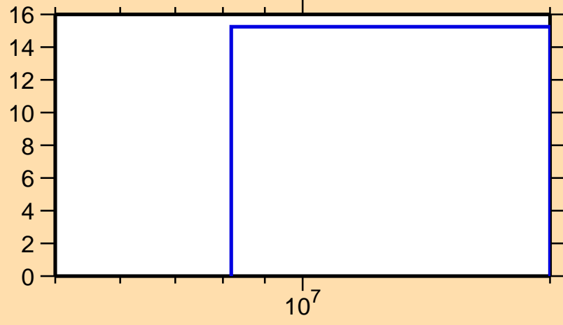
\Delta\sigma/\sigma vs. E for ^{240}\text{Cf}(n,\text{el.})
