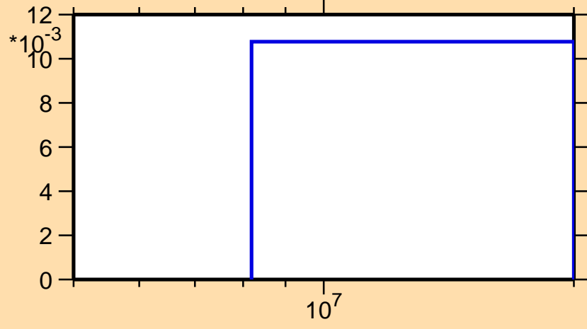
\sigma vs. E for ^{240}\text{Cf}(n,2n)
