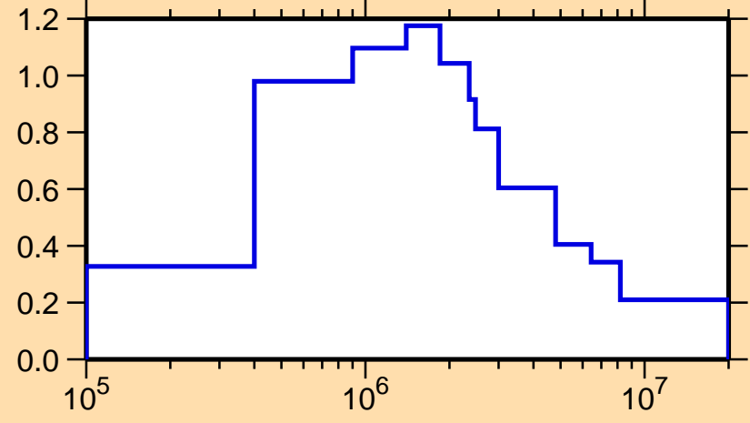
\sigma vs. E for ^{240}\text{Cf}(n,\text{inel.})
