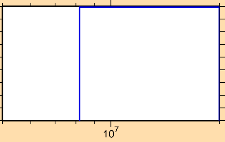
\sigma vs. E for ^{240}\text{Cf}(n,3n)
