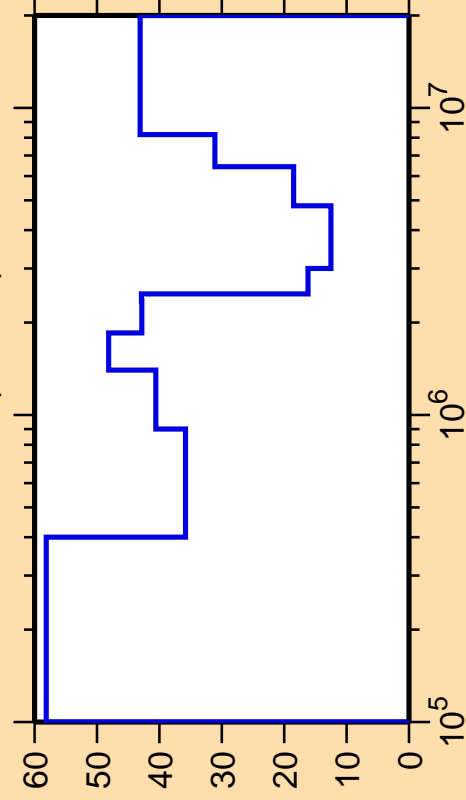
\Delta\sigma/\sigma vs. E for ^{240}\text{Cf}(n,\text{inel.})
