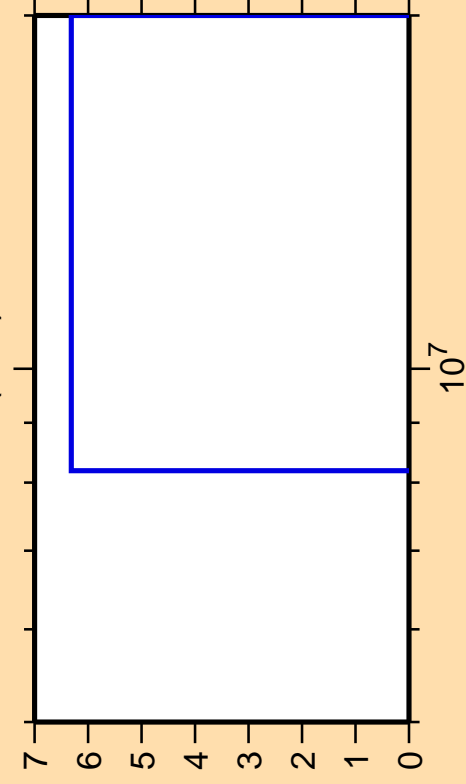
\Delta\sigma/\sigma vs. E for ^{240}\text{Cf}(n,nt)
