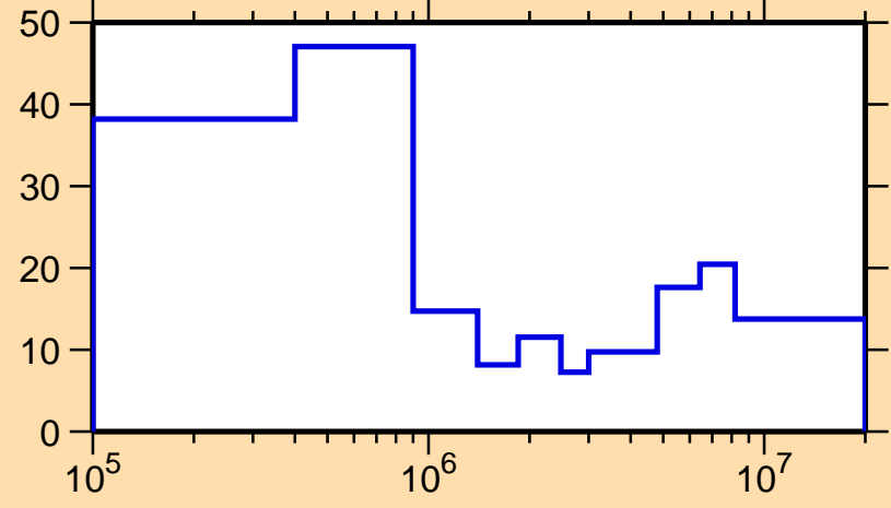
\Delta\sigma/\sigma vs. E for ^{240}\text{Cf}(n,\text{tot.})
