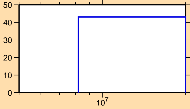
\Delta\sigma/\sigma vs. E for ^{240}\text{Cf}(n,\text{inel.})
