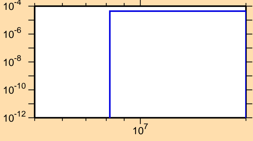
\sigma vs. E for ^{240}\text{Cf}(n,t)
