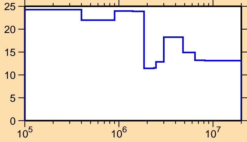
\Delta\sigma/\sigma vs. E for ^{240}\text{Cf}(n,\text{nonel.})
