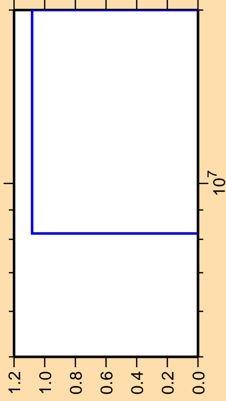
\Delta\sigma/\sigma vs. E for ^{240}\text{Cf} (mt 45)
