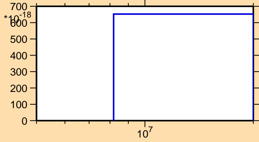
\sigma vs. E for ^{240}\text{Cf}(\text{mt } 34)
