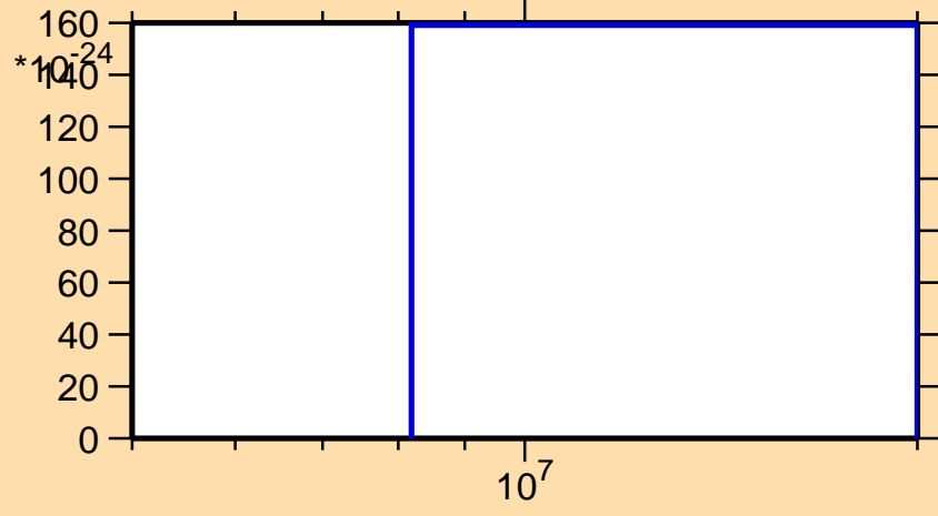
\sigma vs. E for ^{240}\text{Cf}(\text{mt } 42)
