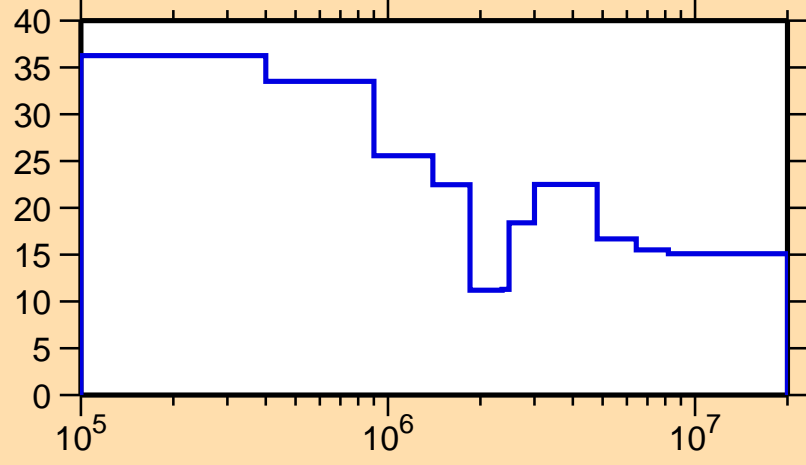
\Delta\sigma/\sigma vs. E for ^{240}\text{Cf}(n,f)
