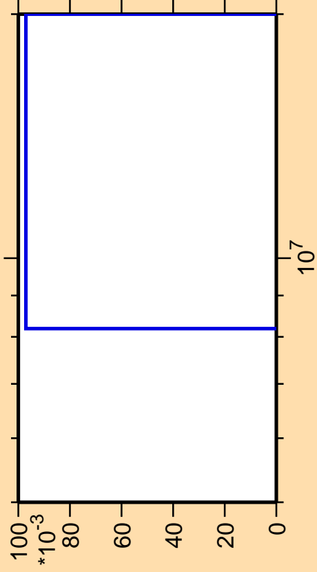
\Delta\sigma/\sigma vs. E for ^{240}\text{Cf}(n,3n\alpha)
