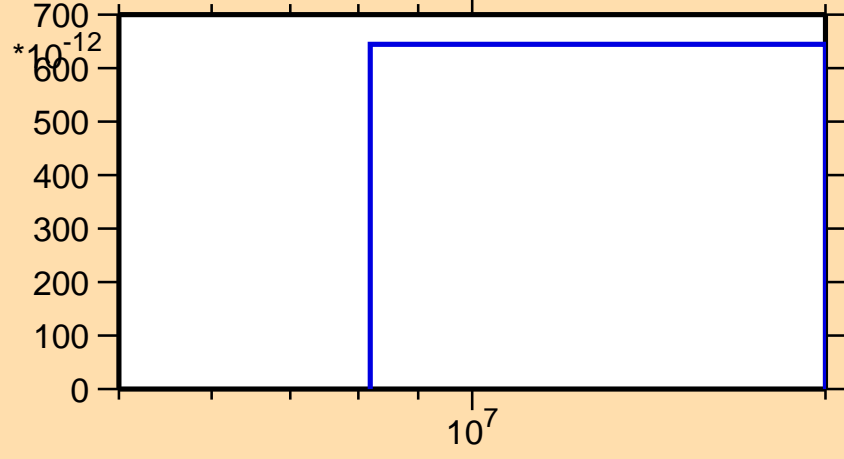
\sigma vs. E for ^{240}\text{Cf}(n,2np)
