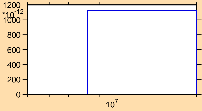
\sigma vs. E for ^{240}\text{Cf}(n,\text{He3})
