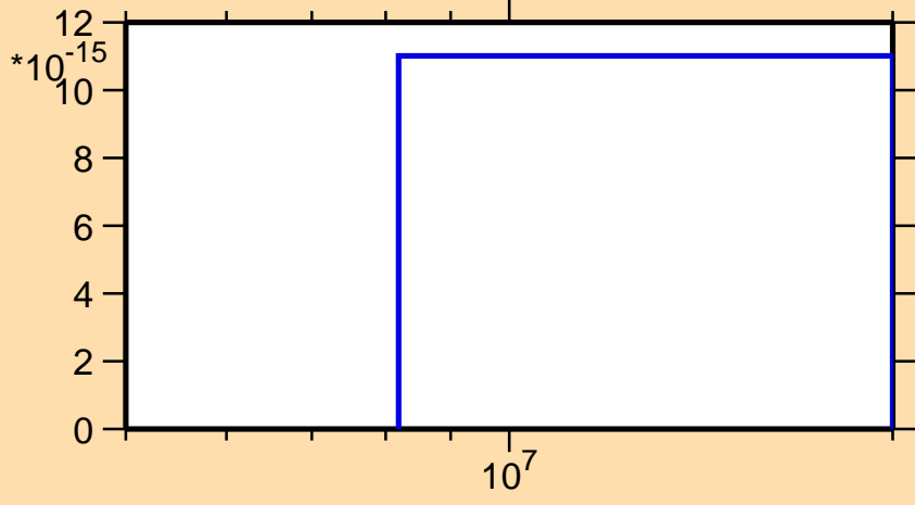
\sigma vs. E for ^{240}\text{Cf}(n,3n\alpha)
