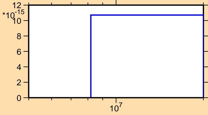
\sigma vs. E for ^{240}\text{Cf}(n,\text{pd})
