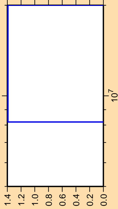
\Delta\sigma/\sigma vs. E for ^{240}\text{Cf}(\text{mt117})
