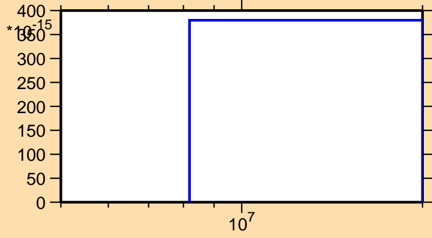
\sigma vs. E for ^{240}\text{Cf}(\text{mt117})
