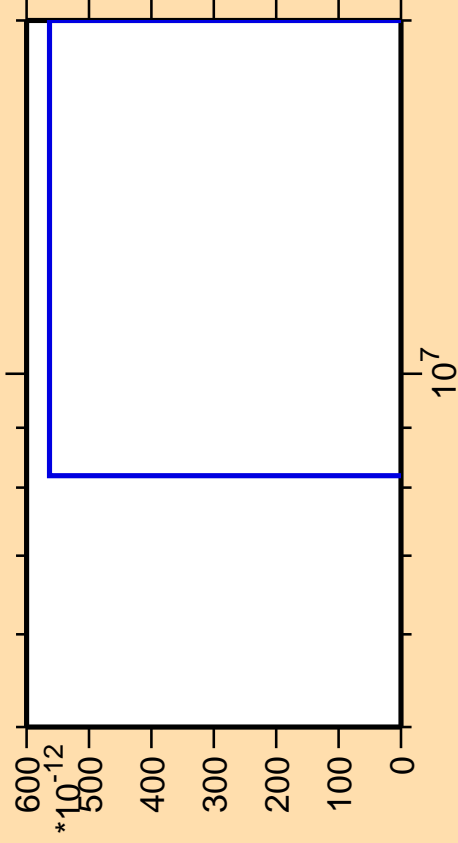
\Delta\sigma/\sigma vs. E for ^{240}\text{Cf}(\text{mt } 42)
