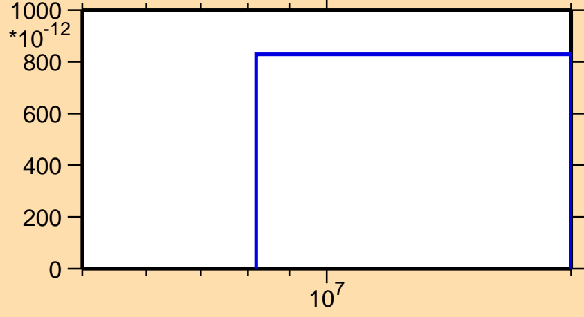
\sigma vs. E for ^{240}\text{Cf}(n,2n\alpha)
