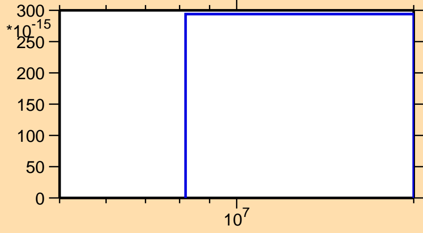
\sigma vs. E for ^{240}\text{Cf} (mt 45)
