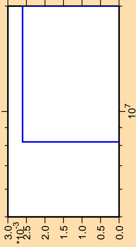
\Delta\sigma/\sigma vs. E for ^{240}\text{Cf}(\text{mt } 34)
