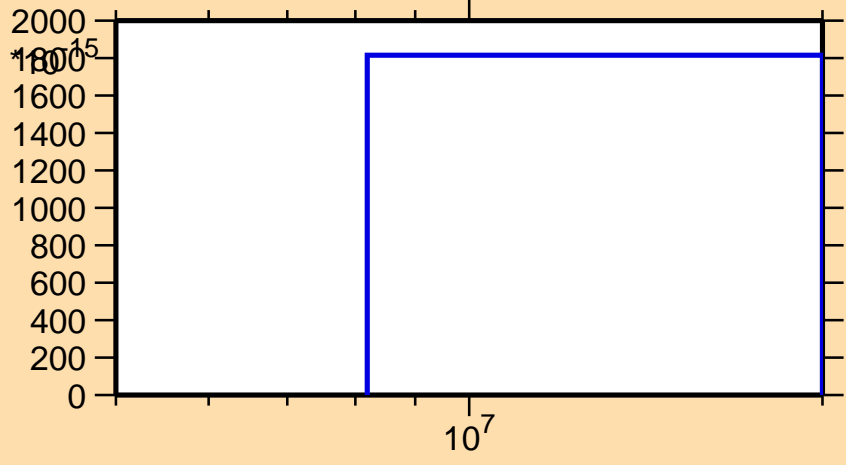
\sigma vs. E for ^{240}\text{Cf}(n,nt)
