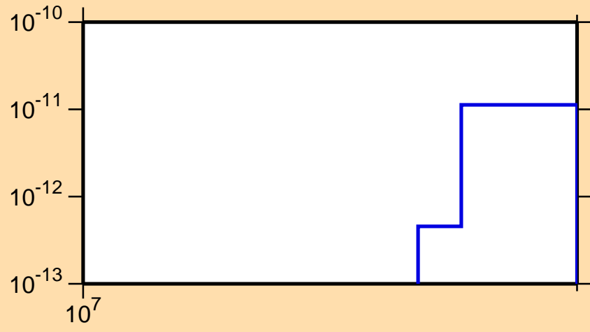
\sigma vs. E for ^{241}\text{Cf} (mt 34)
